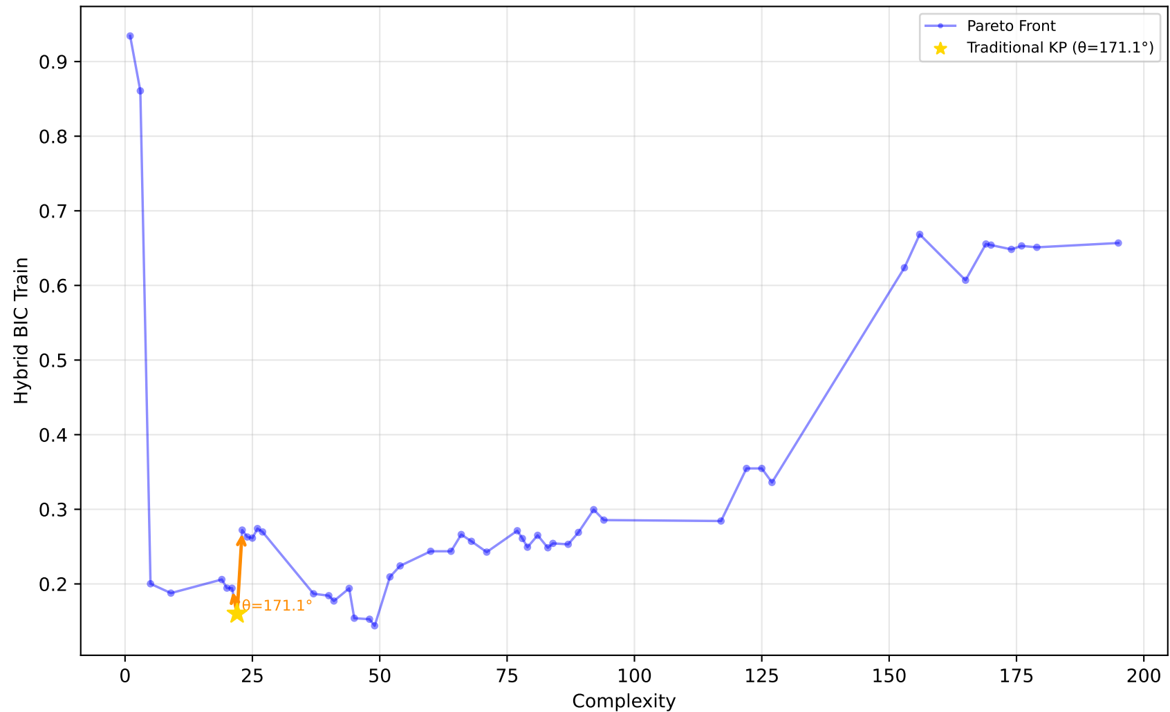
712_chscase_geyser1 - Run 2 - SVP - Hybrid BIC Train \lambda_1=0.00 , \lambda_2=1.00 , \lambda_3=1.00 | Difficulty: 1.00 | Method: hmr
