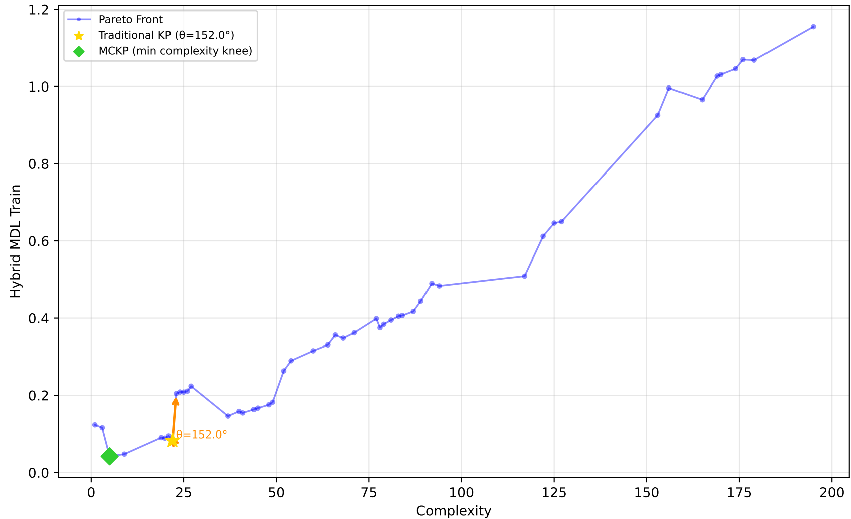
712_chscase_geyser1 - Run 2 - SVP - Hybrid MDL Train \lambda_1=0.00, \lambda_2=1.00, \lambda_3=1.00 | Difficulty: 1.00 | Method: hmr
