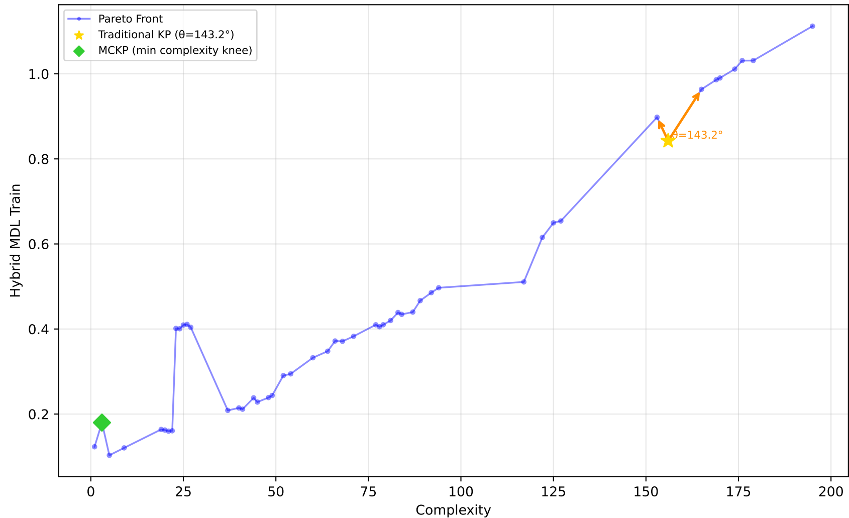
712_chscase_geyser1 - Run 2 - SVP - Hybrid MDL Train \lambda_1=1.00, \lambda_2=1.00, \lambda_3=0.00 | Difficulty: 1.00 | Method: hmr
