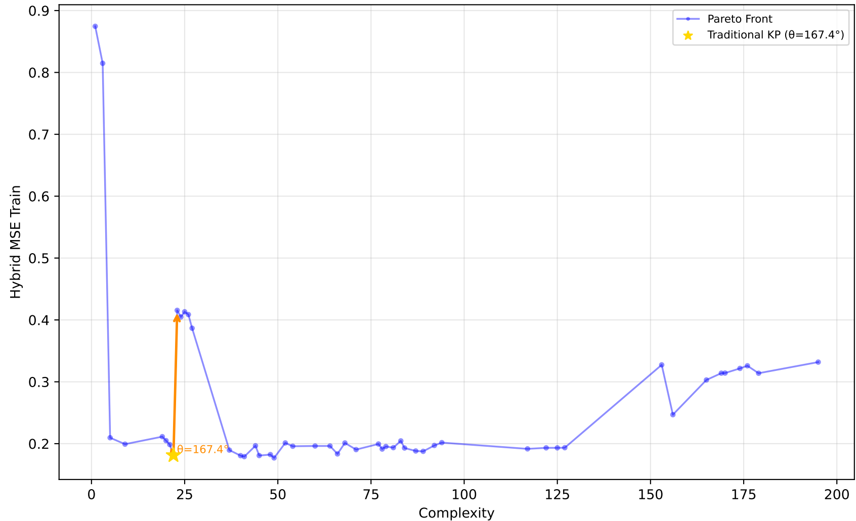
712_chscase_geyser1 - Run 2 - SVP - Hybrid MSE Train \lambda_1=1.00, \lambda_2=1.00, \lambda_3=0.00 | Difficulty: 1.00 | Method: hmr
