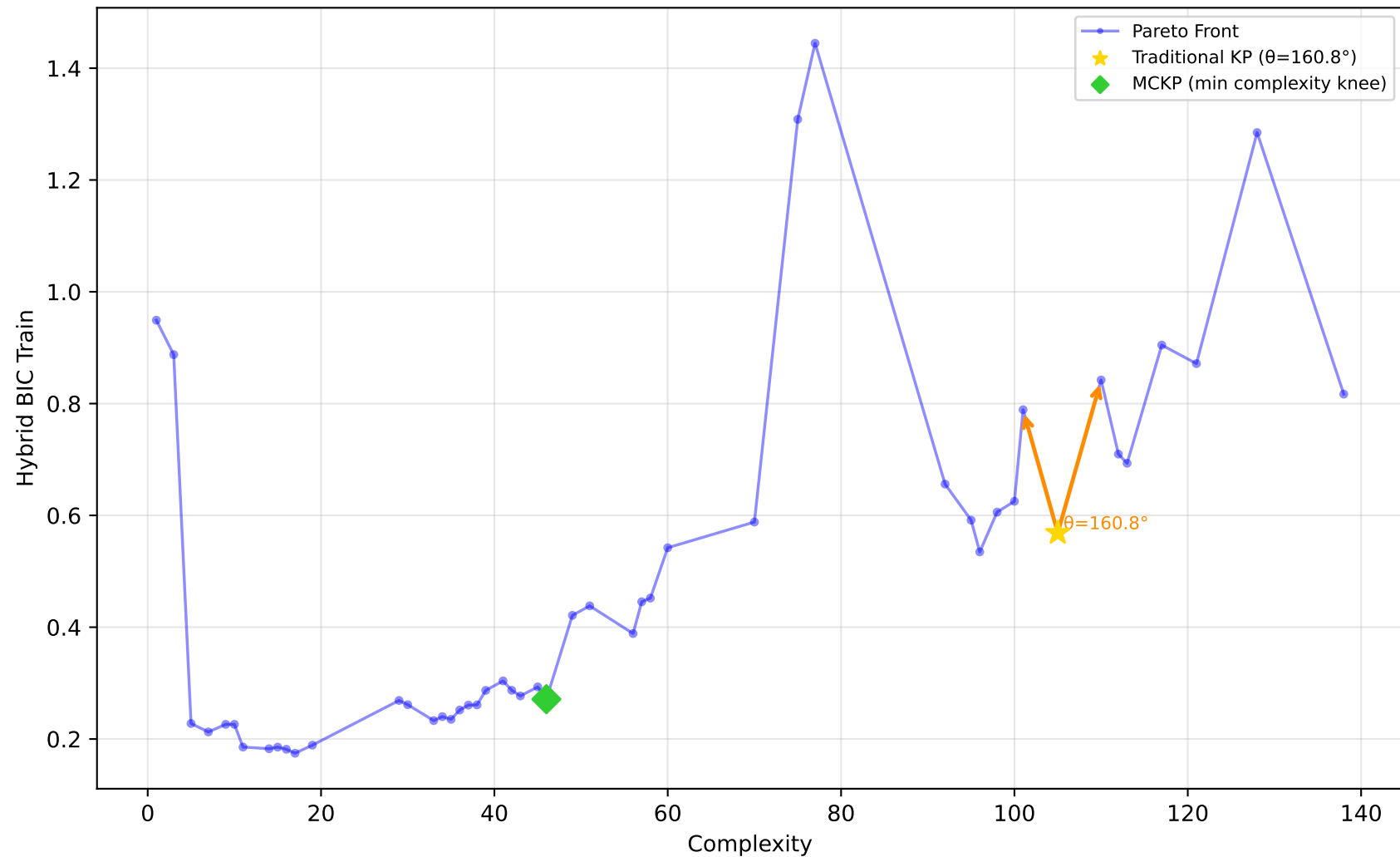
712_chscase_geyser1 - Run 30 - MVP - Hybrid BIC Train \lambda_1=0.20, \lambda_2=1.00, \lambda_3=1.00 | Difficulty: 0.37 | Method: mckp
