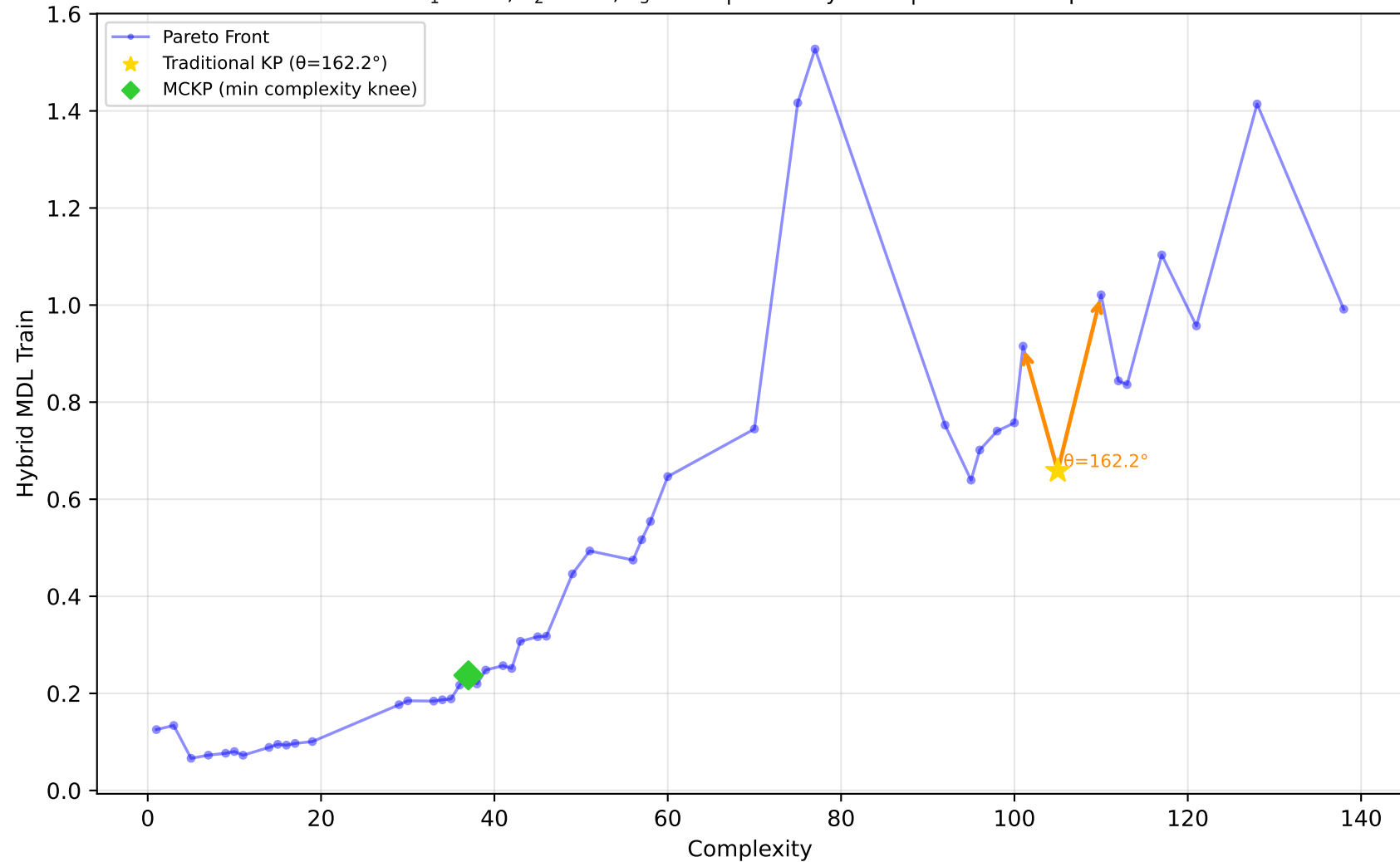
712_chscase_geyser1 - Run 30 - MVP - Hybrid MDL Train \lambda_1=0.20, \lambda_2=1.00, \lambda_3=1.00 | Difficulty: 0.37 | Method: mckp
