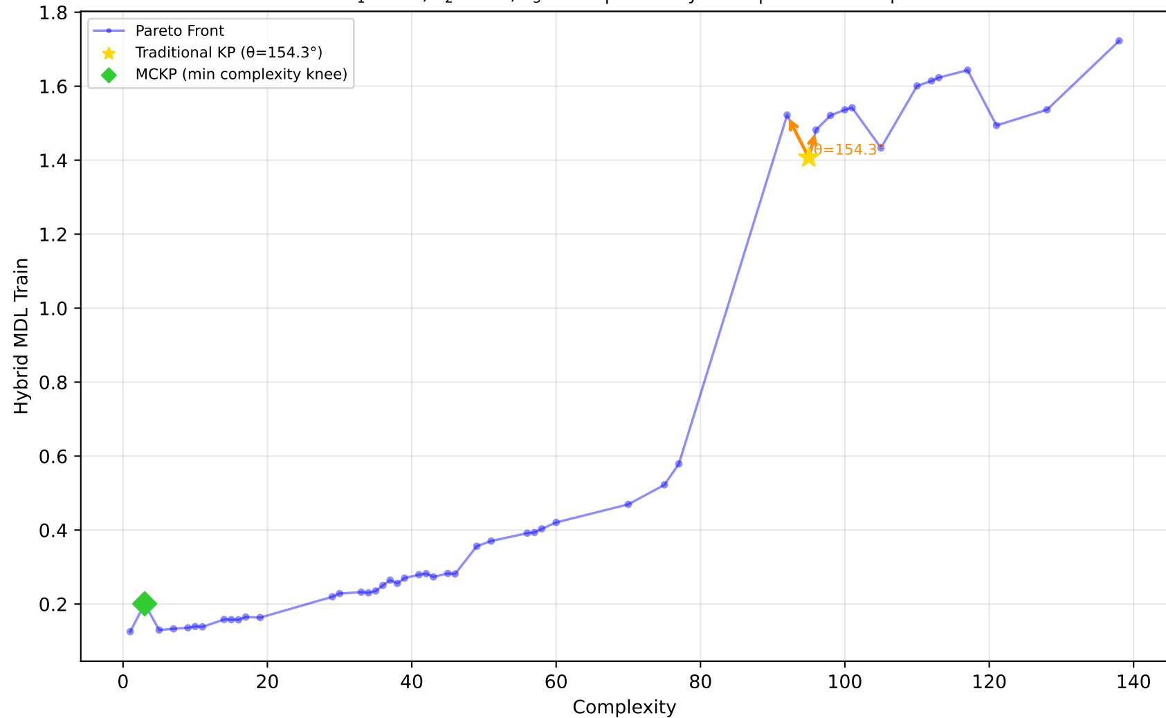
712_chscase_geyser1 - Run 30 - SVP - Hybrid MDL Train \lambda_1=1.00, \lambda_2=1.00, \lambda_3=0.00 | Difficulty: 0.37 | Method: mckp
