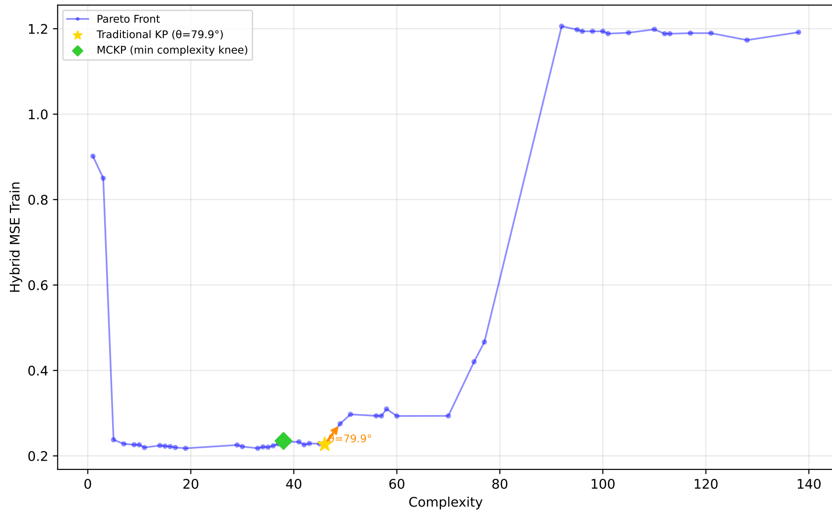
712_chscase_geyser1 - Run 30 - SVP - Hybrid MSE Train \lambda_1=1.00, \lambda_2=1.00, \lambda_3=0.00 | Difficulty: 0.37 | Method: mckp
