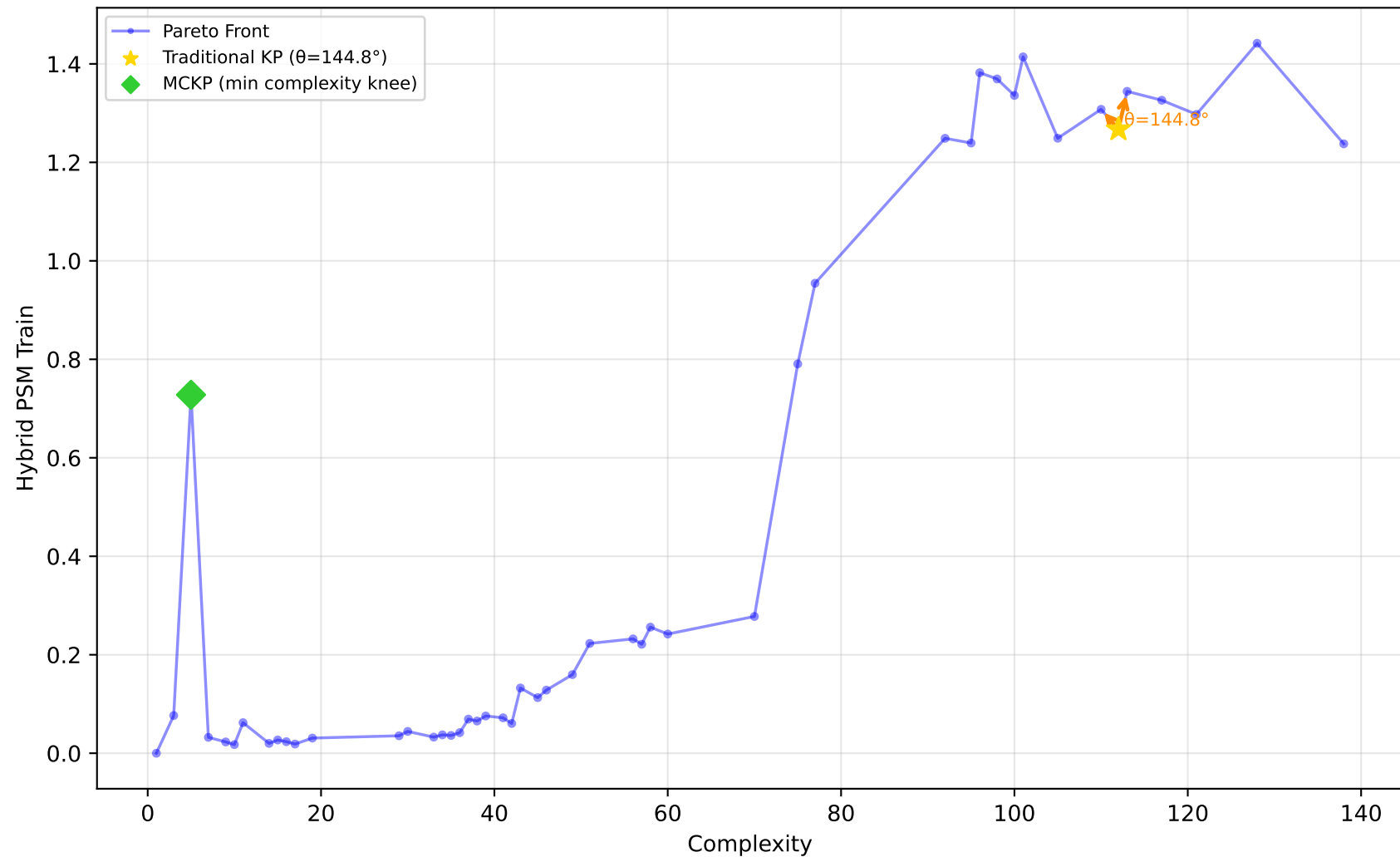
712_chscase_geyser1 - Run 30 - SVP - Hybrid PSM Train \lambda_1=0.00 , \lambda_2=1.00 , \lambda_3=1.00 | Difficulty: 0.37 | Method: mckp
