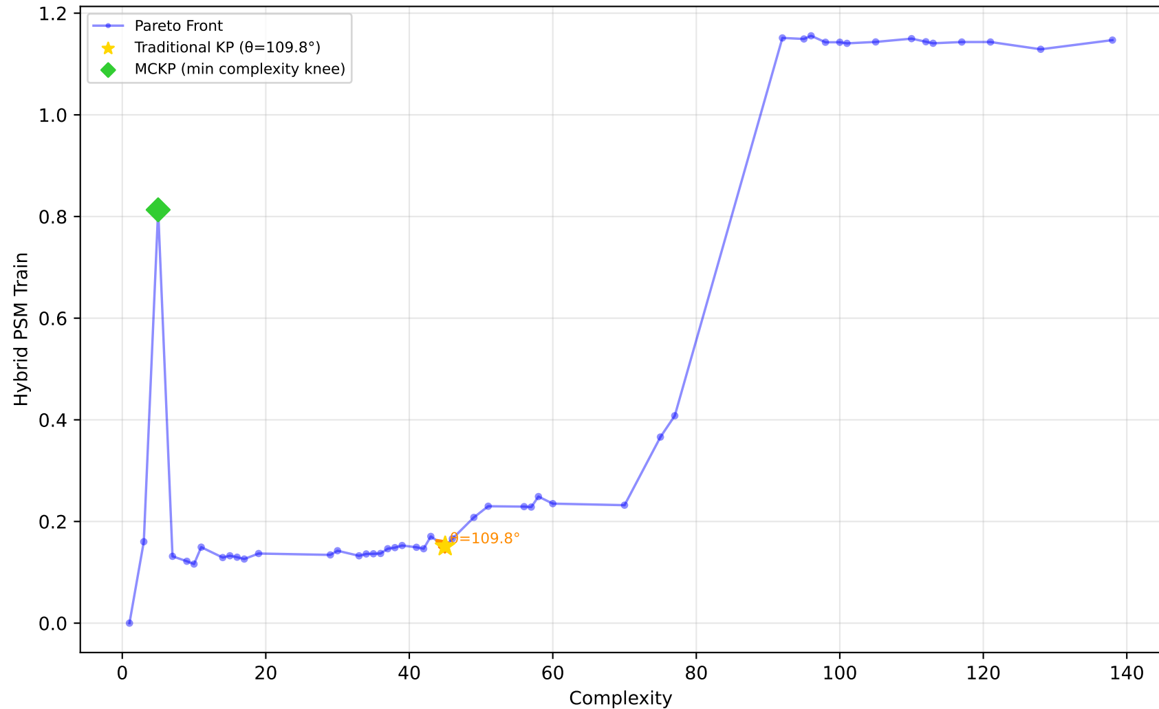
712_chscase_geyser1 - Run 30 - SVP - Hybrid PSM Train \lambda_1=1.00, \lambda_2=1.00, \lambda_3=0.00 | Difficulty: 0.37 | Method: mckp
