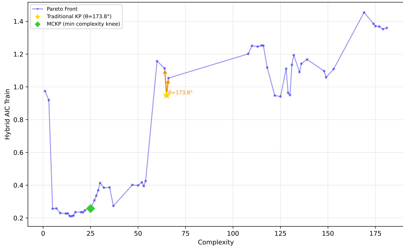
712_chscase_geyser1 - Run 3 - MVP - Hybrid AIC Train \lambda_1=0.20 , \lambda_2=1.00 , \lambda_3=1.00 | Difficulty: 0.41 | Method: mckp
