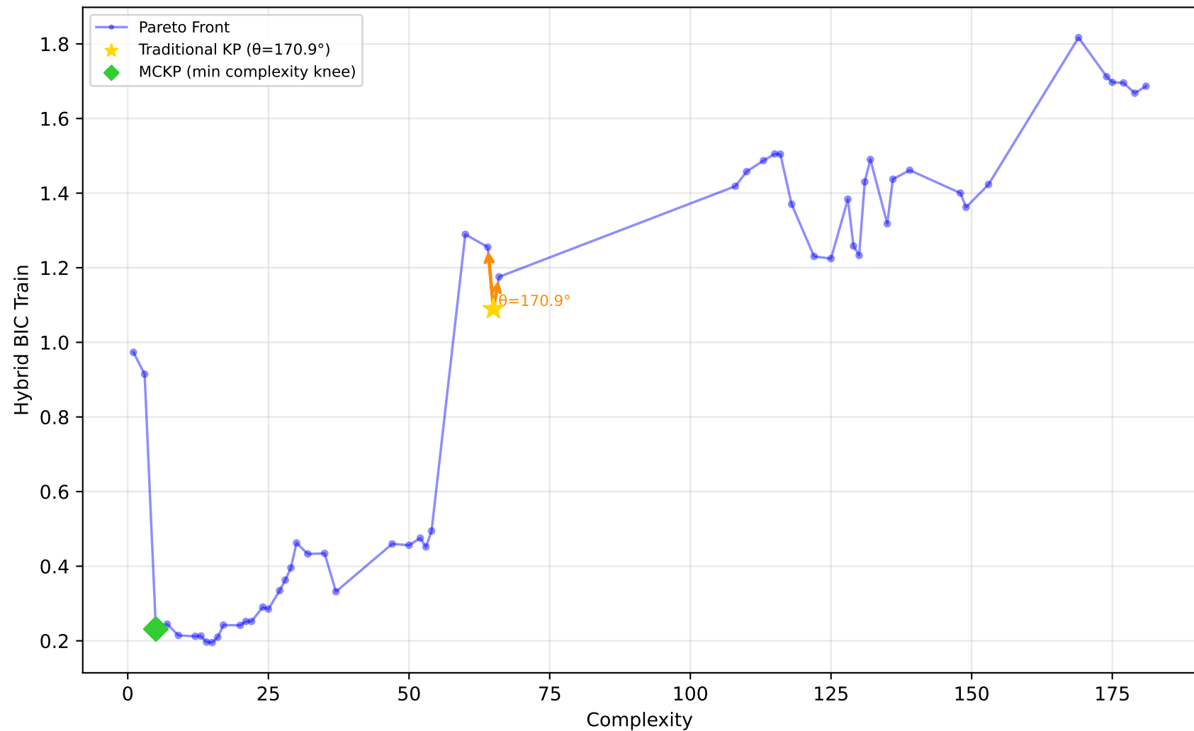
712_chscase_geyser1 - Run 3 - MVP - Hybrid BIC Train \lambda_1=0.20 , \lambda_2=1.00 , \lambda_3=1.00 | Difficulty: 0.41 | Method: mckp
