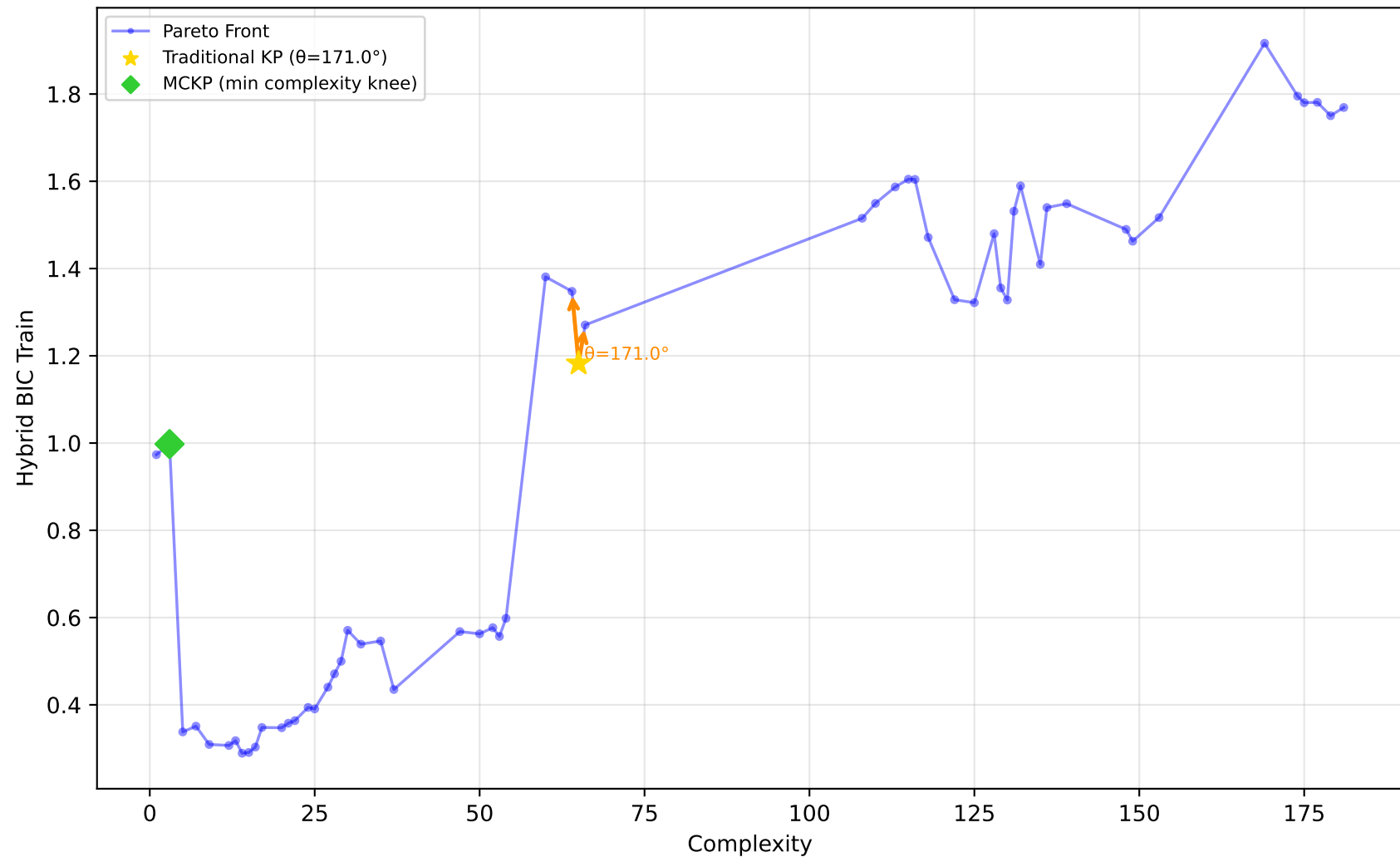
712_chscase_geyser1 - Run 3 - MVP - Hybrid BIC Train \lambda_1=1.00, \lambda_2=1.00, \lambda_3=1.00 | Difficulty: 0.41 | Method: mckp
