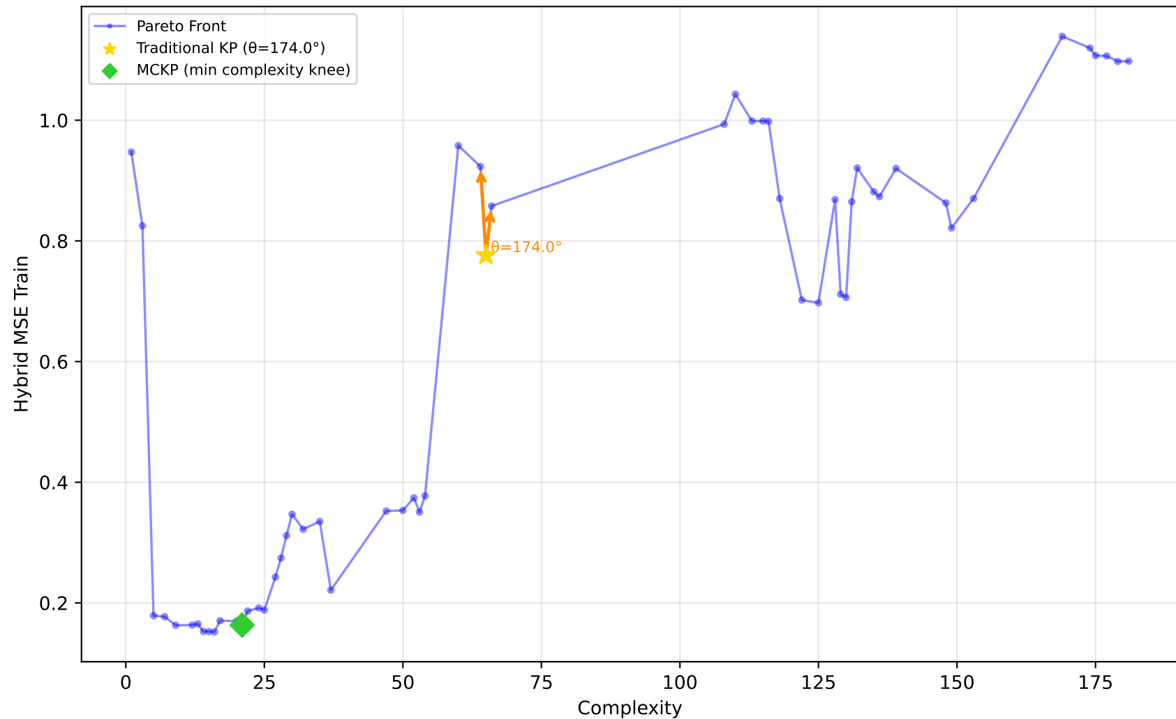
712_chscase_geyser1 - Run 3 - MVP - Hybrid MSE Train \lambda_1=0.20, \lambda_2=1.00, \lambda_3=1.00 | Difficulty: 0.41 | Method: mckp
