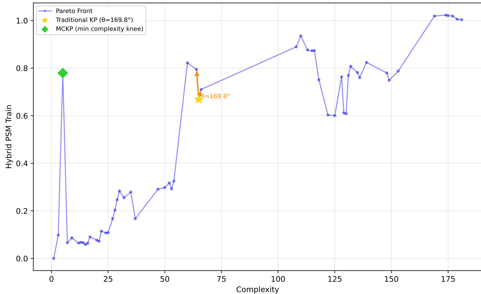
712_chscase_geyser1 - Run 3 - MVP - Hybrid PSM Train \lambda_1=0.20, \lambda_2=1.00, \lambda_3=1.00 | Difficulty: 0.41 | Method: mckp
