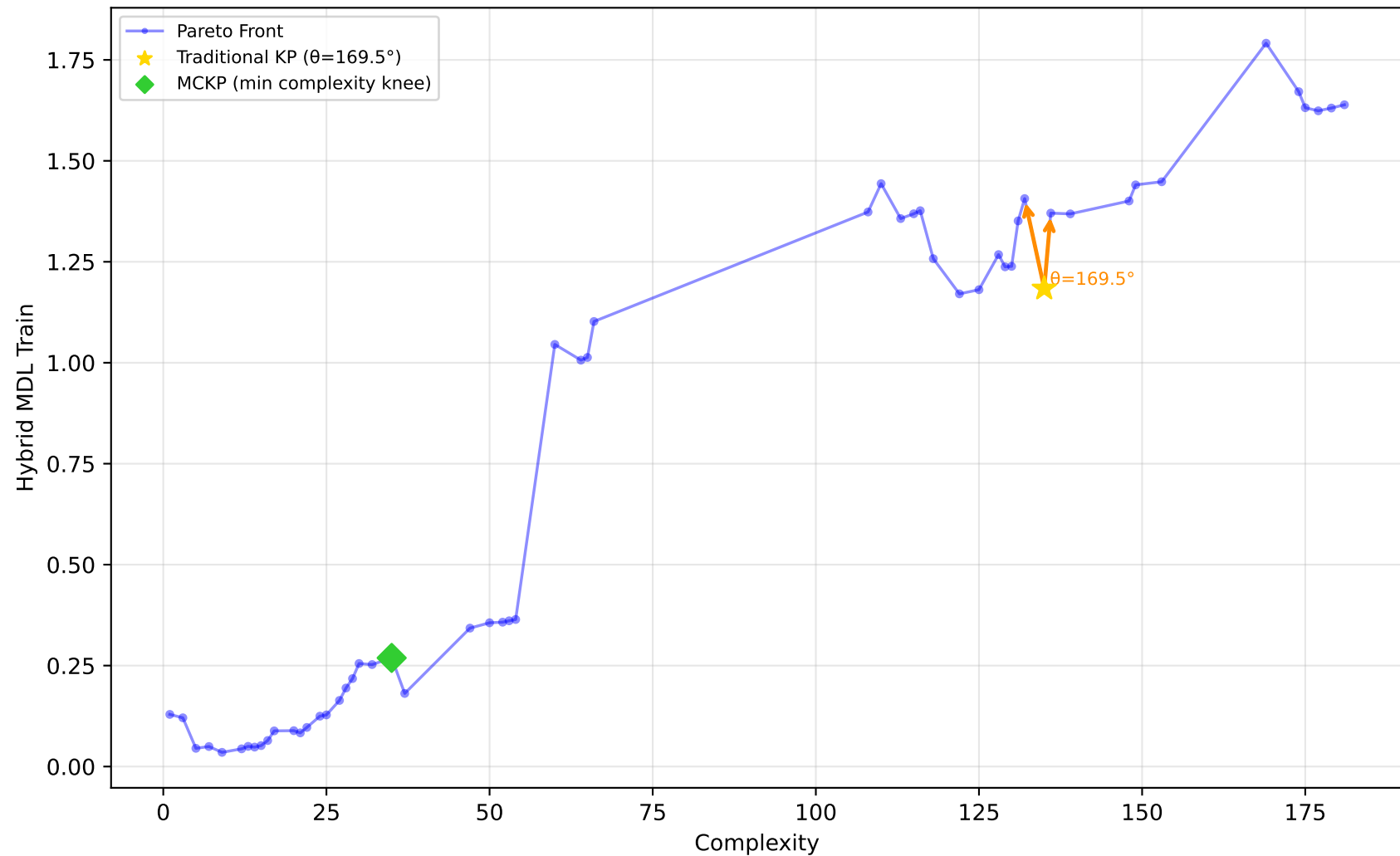
712_chscase_geyser1 - Run 3 - SVP - Hybrid MDL Train \lambda_1=0.00, \lambda_2=1.00, \lambda_3=1.00 | Difficulty: 0.41 | Method: mckp
