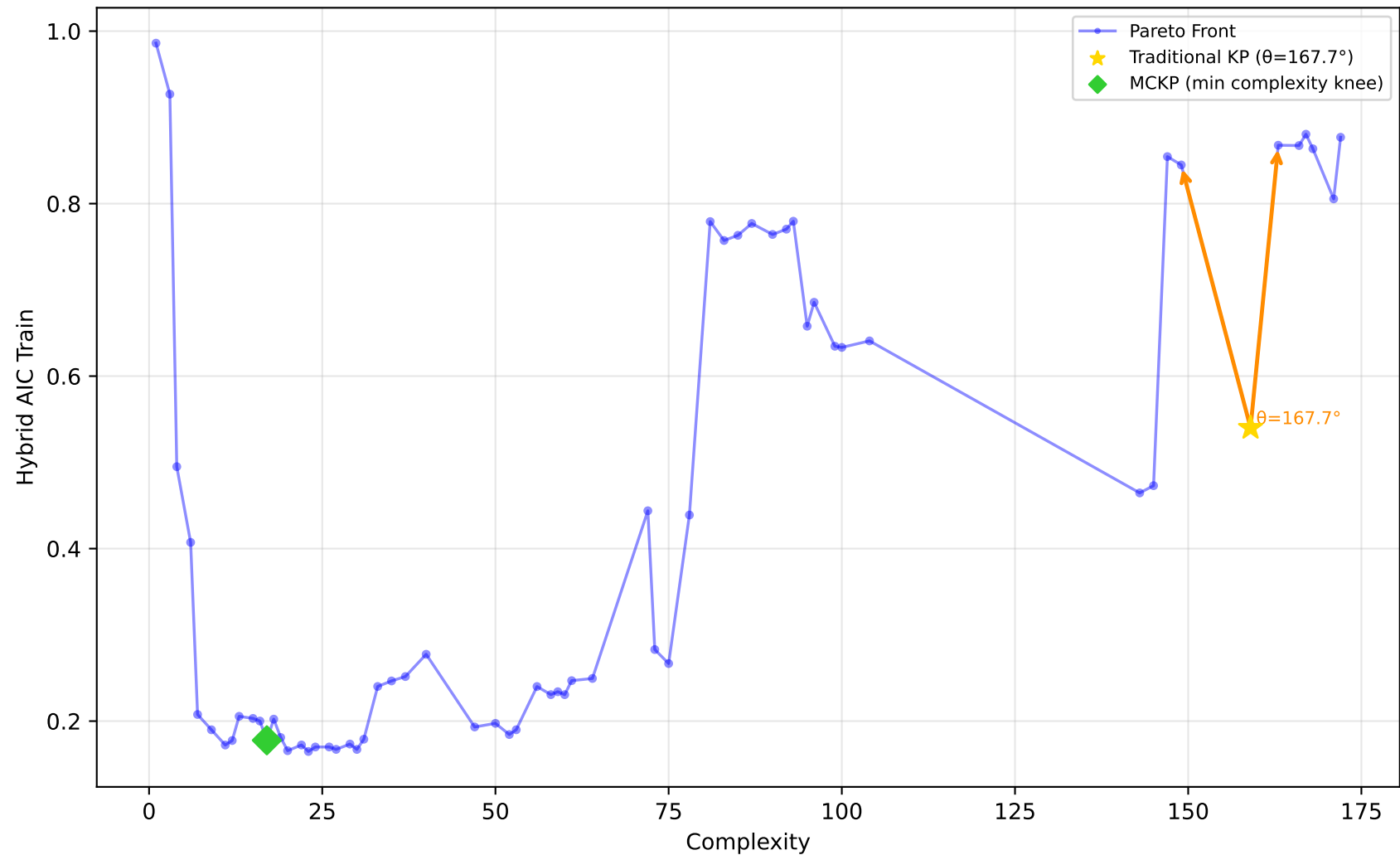
712_chscase_geyser1 - Run 4 - MVP - Hybrid AIC Train \lambda_1=0.20 , \lambda_2=1.00 , \lambda_3=1.00 | Difficulty: 0.48 | Method: mckp
