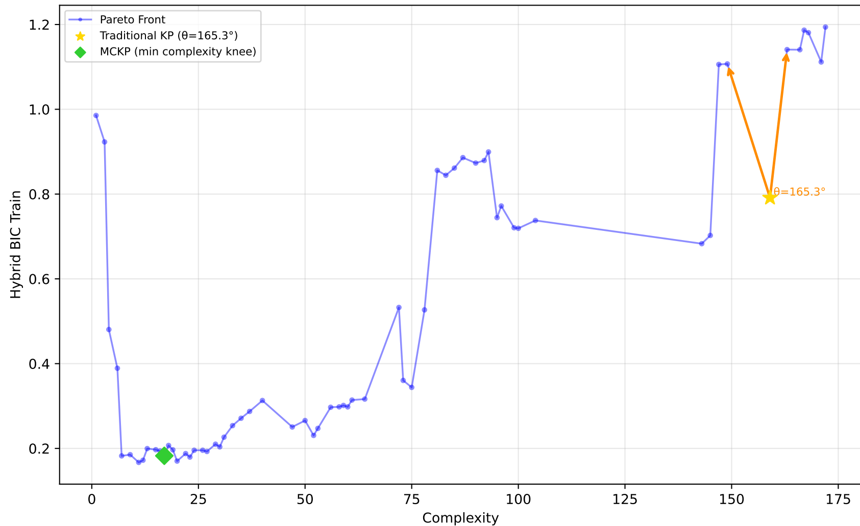
712_chscase_geyser1 - Run 4 - MVP - Hybrid BIC Train \lambda_1=0.20 , \lambda_2=1.00 , \lambda_3=1.00 | Difficulty: 0.48 | Method: mckp
