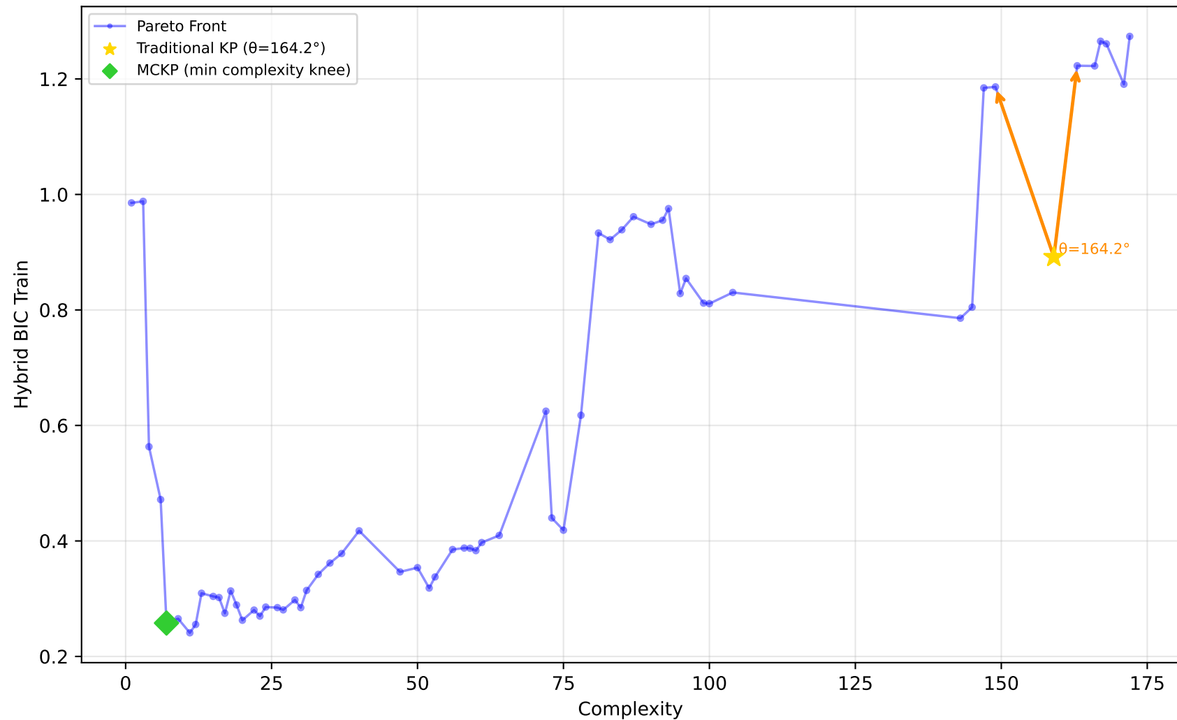
712_chscase_geyser1 - Run 4 - MVP - Hybrid BIC Train \lambda_1=1.00, \lambda_2=1.00, \lambda_3=1.00 | Difficulty: 0.48 | Method: mckp
