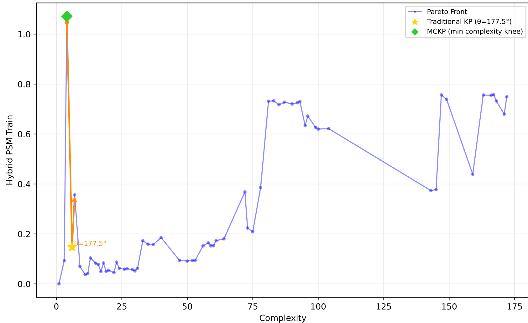
712_chscase_geyser1 - Run 4 - MVP - Hybrid PSM Train \lambda_1=0.20, \lambda_2=1.00, \lambda_3=1.00 | Difficulty: 0.48 | Method: mckp
