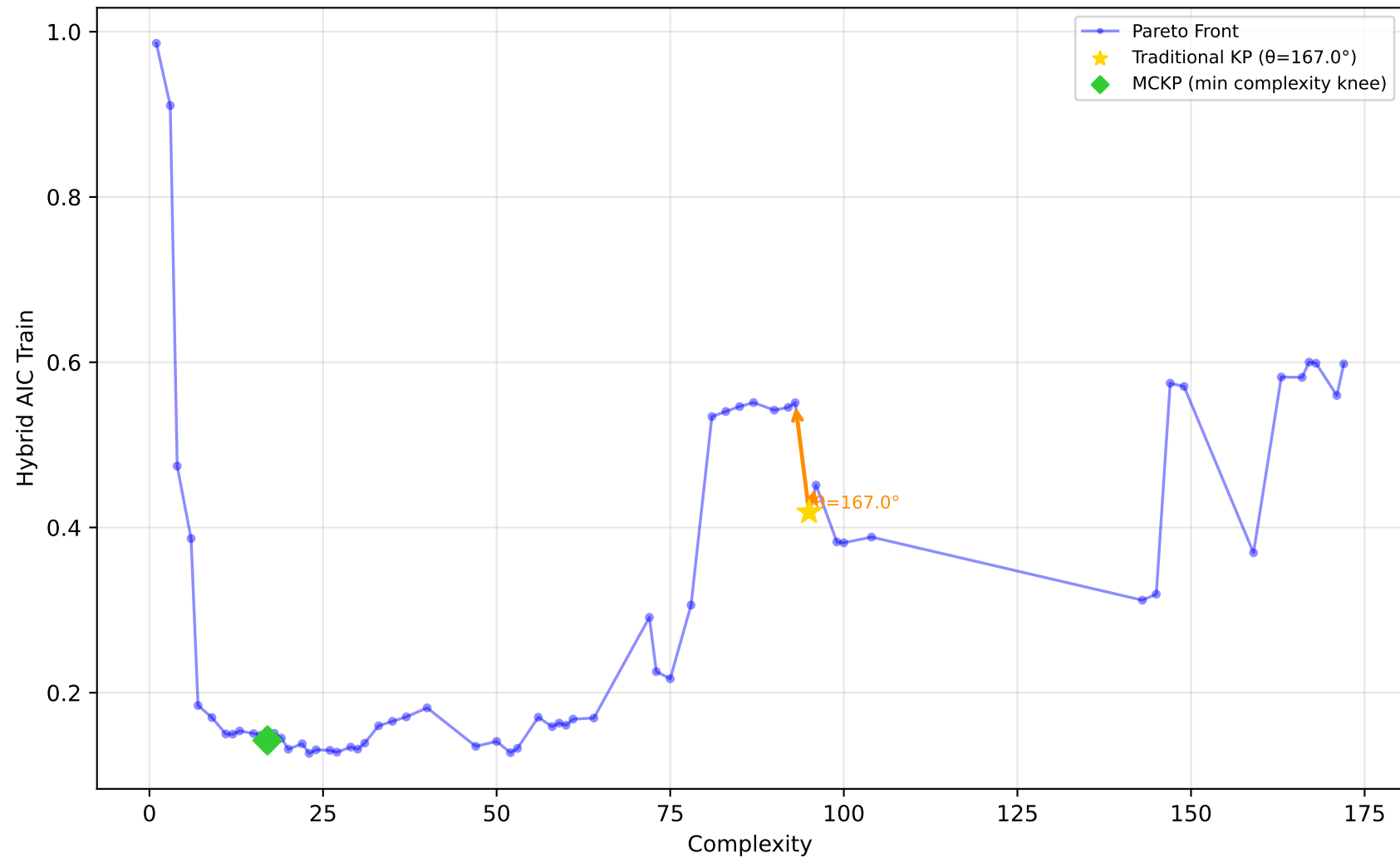
712_chscase_geyser1 - Run 4 - SVP - Hybrid AIC Train \lambda_1=0.00 , \lambda_2=1.00 , \lambda_3=1.00 | Difficulty: 0.48 | Method: mckp
