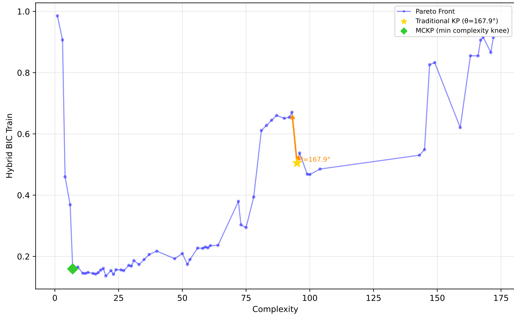
712_chscase_geyser1 - Run 4 - SVP - Hybrid BIC Train \lambda_1=0.00 , \lambda_2=1.00 , \lambda_3=1.00 | Difficulty: 0.48 | Method: mckp
