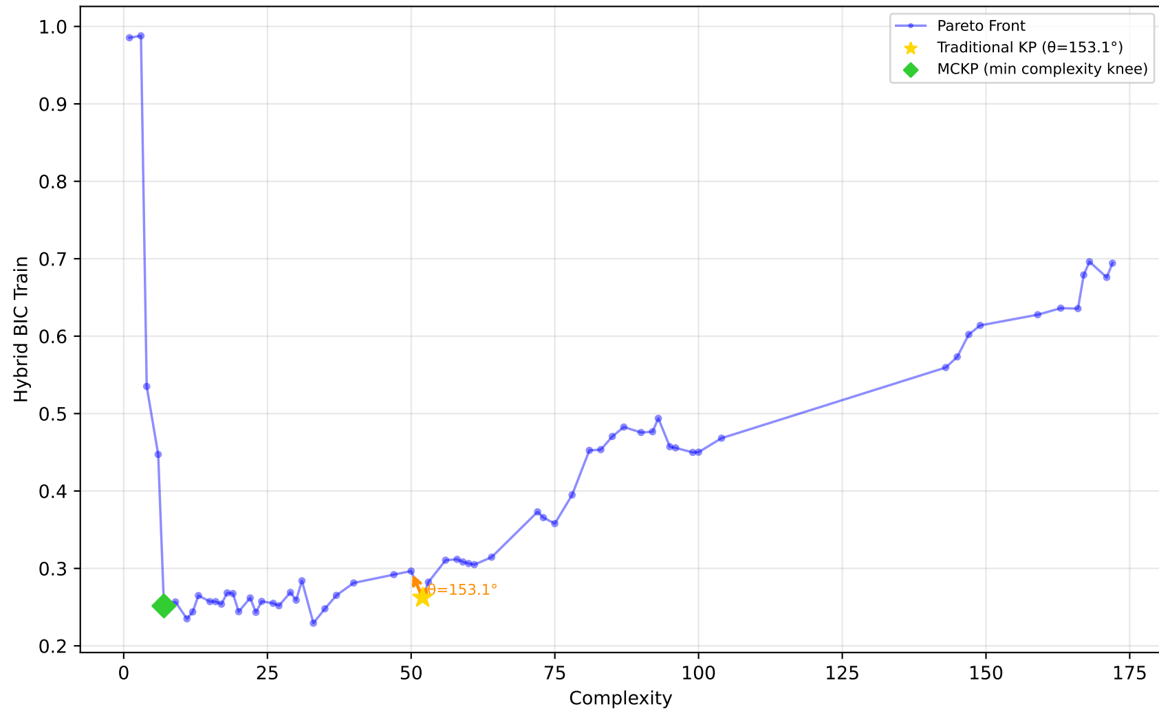
712_chscase_geyser1 - Run 4 - SVP - Hybrid BIC Train \lambda_1=1.00, \lambda_2=1.00, \lambda_3=0.00 | Difficulty: 0.48 | Method: mckp
