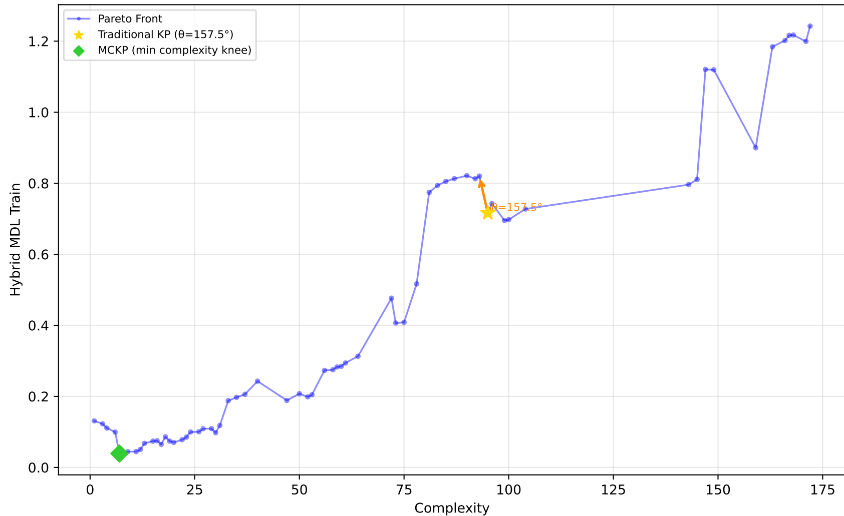
712_chscase_geyser1 - Run 4 - SVP - Hybrid MDL Train \lambda_1=0.00, \lambda_2=1.00, \lambda_3=1.00 | Difficulty: 0.48 | Method: mckp
