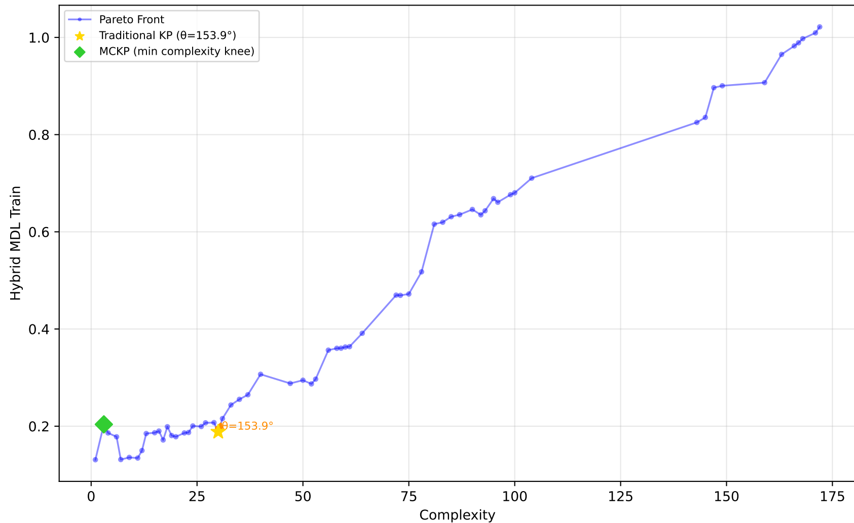
712_chscase_geyser1 - Run 4 - SVP - Hybrid MDL Train \lambda_1=1.00, \lambda_2=1.00, \lambda_3=0.00 | Difficulty: 0.48 | Method: mckp
