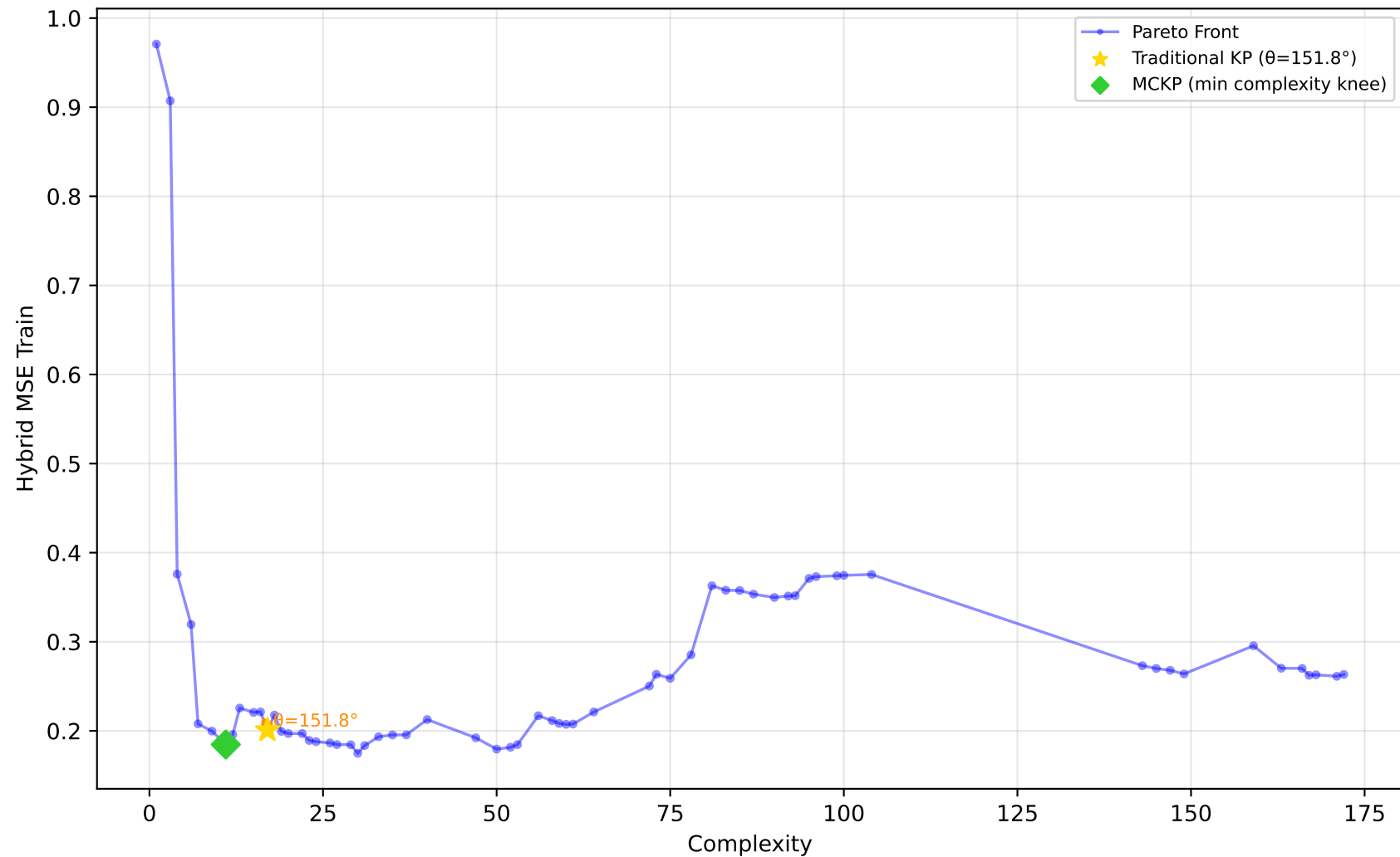
712_chscase_geyser1 - Run 4 - SVP - Hybrid MSE Train \lambda_1=1.00, \lambda_2=1.00, \lambda_3=0.00 | Difficulty: 0.48 | Method: mckp
