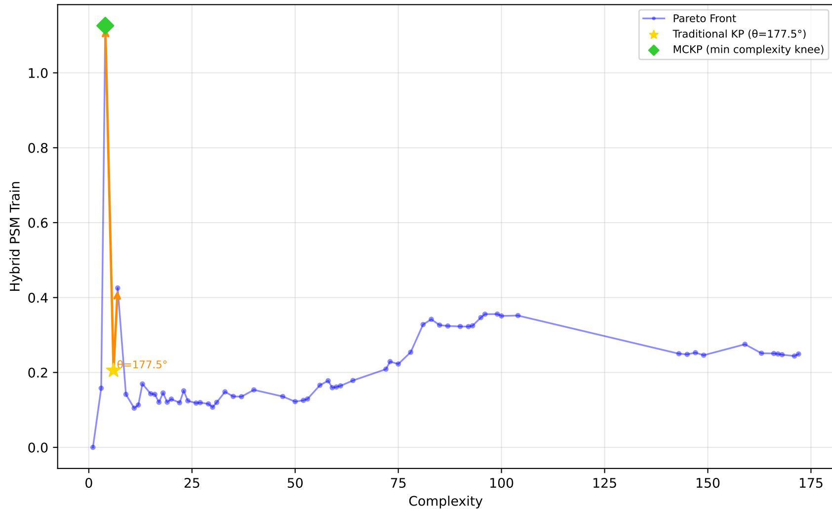
712_chscase_geyser1 - Run 4 - SVP - Hybrid PSM Train \lambda_1=1.00, \lambda_2=1.00, \lambda_3=0.00 | Difficulty: 0.48 | Method: mckp
