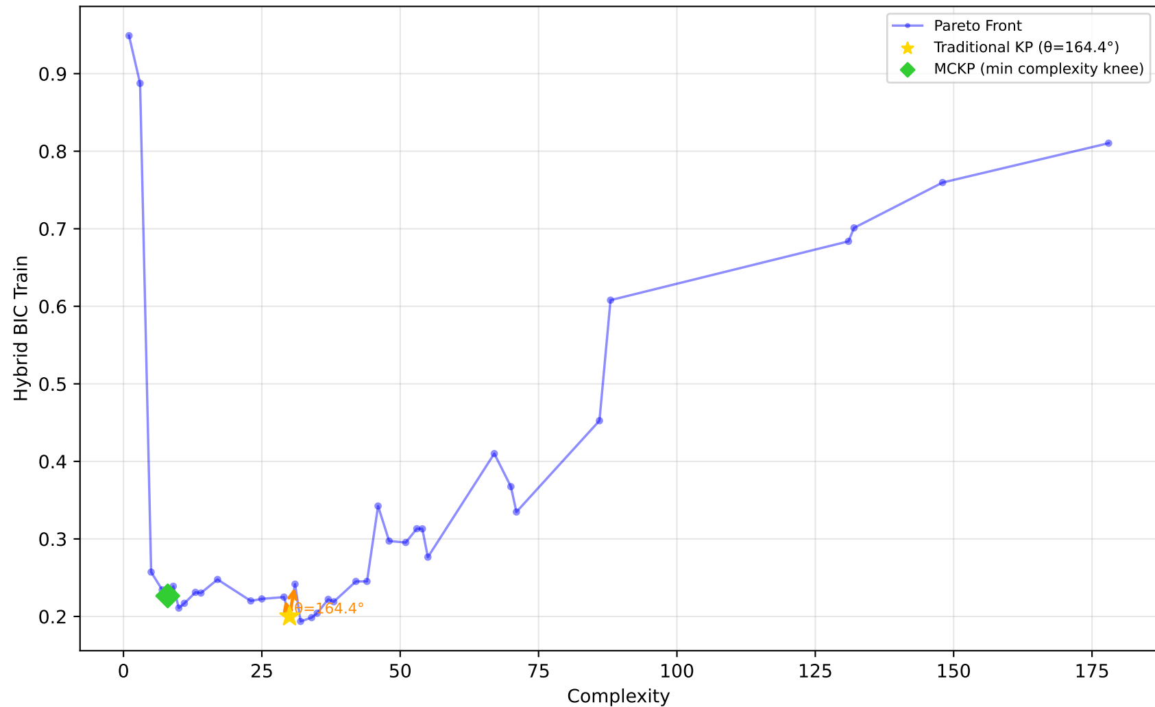
712_chscase_geyser1 - Run 5 - MVP - Hybrid BIC Train \lambda_1=0.20 , \lambda_2=1.00 , \lambda_3=1.00 | Difficulty: 0.92 | Method: hmr
