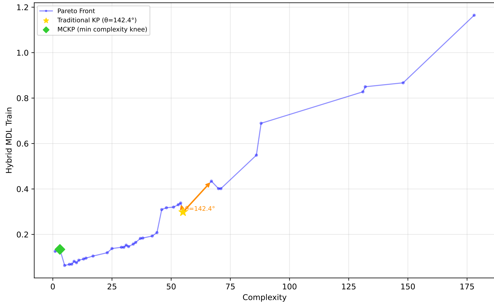
712_chscase_geyser1 - Run 5 - MVP - Hybrid MDL Train \lambda_1=0.20, \lambda_2=1.00, \lambda_3=1.00 | Difficulty: 0.92 | Method: hmr
