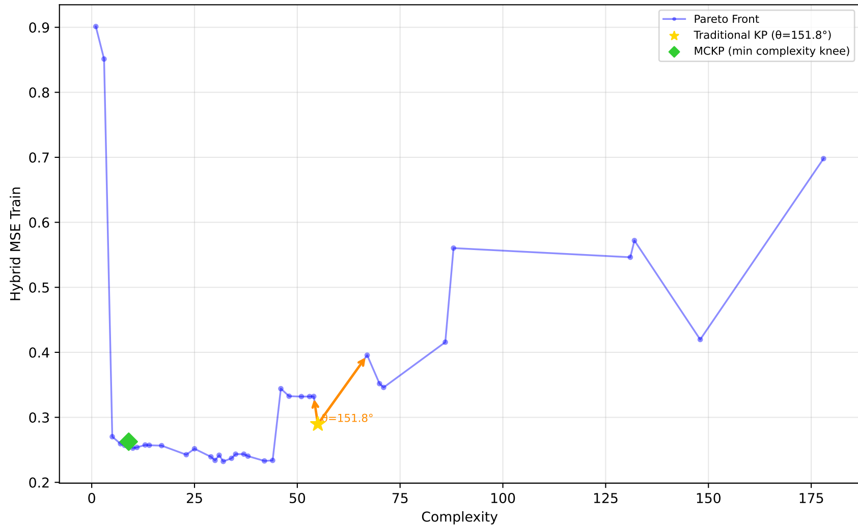
712_chscase_geyser1 - Run 5 - MVP - Hybrid MSE Train \lambda_1=1.00, \lambda_2=1.00, \lambda_3=1.00 | Difficulty: 0.92 | Method: hmr
