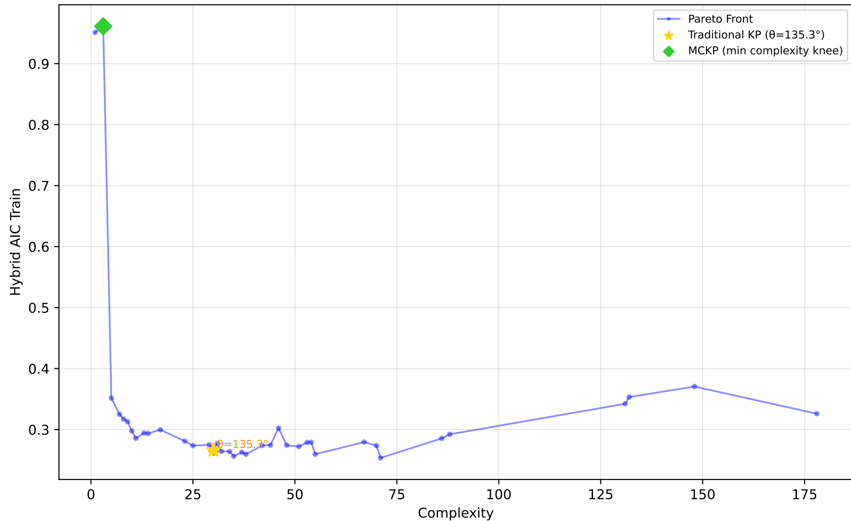
712_chscase_geyser1 - Run 5 - SVP - Hybrid AIC Train \lambda_1=1.00, \lambda_2=1.00, \lambda_3=0.00 | Difficulty: 0.92 | Method: hmr
