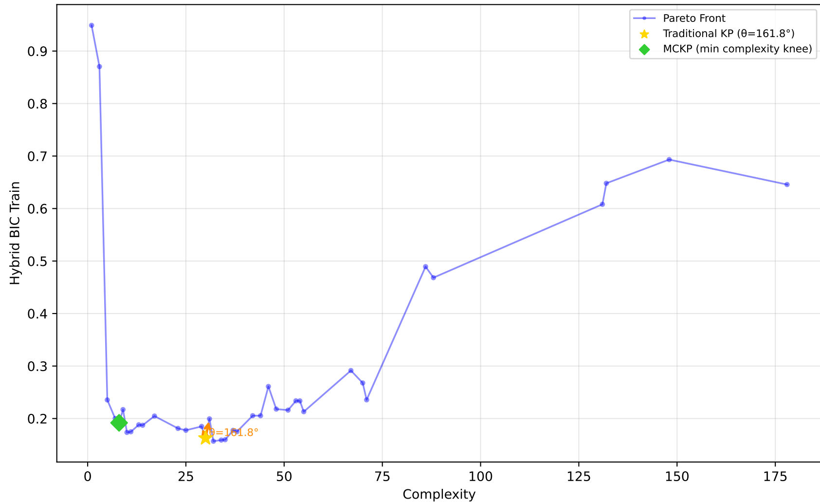
712_chscase_geyser1 - Run 5 - SVP - Hybrid BIC Train \lambda_1=0.00, \lambda_2=1.00, \lambda_3=1.00 | Difficulty: 0.92 | Method: hmr
