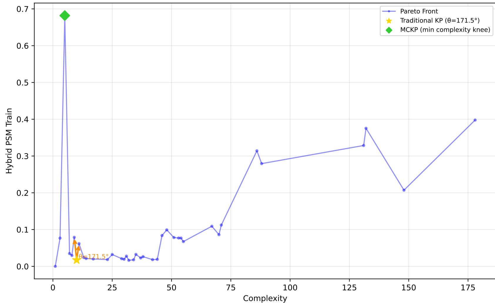
712_chscase_geyser1 - Run 5 - SVP - Hybrid PSM Train \lambda_1=0.00, \lambda_2=1.00, \lambda_3=1.00 | Difficulty: 0.92 | Method: hmr
