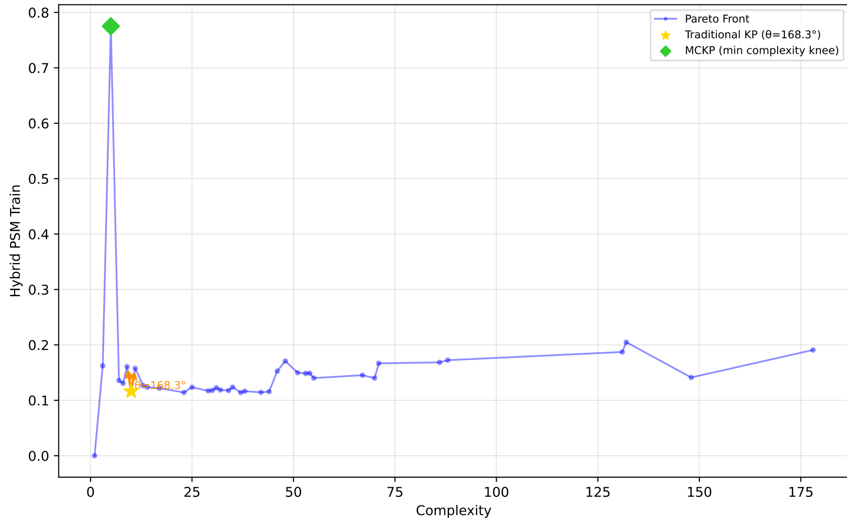
712_chscase_geyser1 - Run 5 - SVP - Hybrid PSM Train \lambda_1=1.00, \lambda_2=1.00, \lambda_3=0.00 | Difficulty: 0.92 | Method: hmr
