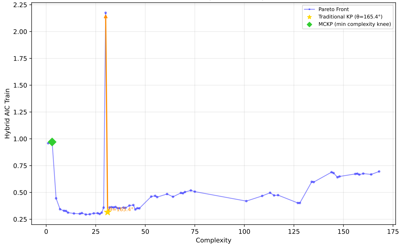
712_chscase_geyser1 - Run 6 - MVP - Hybrid AIC Train \lambda_1=1.00 , \lambda_2=1.00 , \lambda_3=1.00 | Difficulty: 1.00 | Method: hmr
