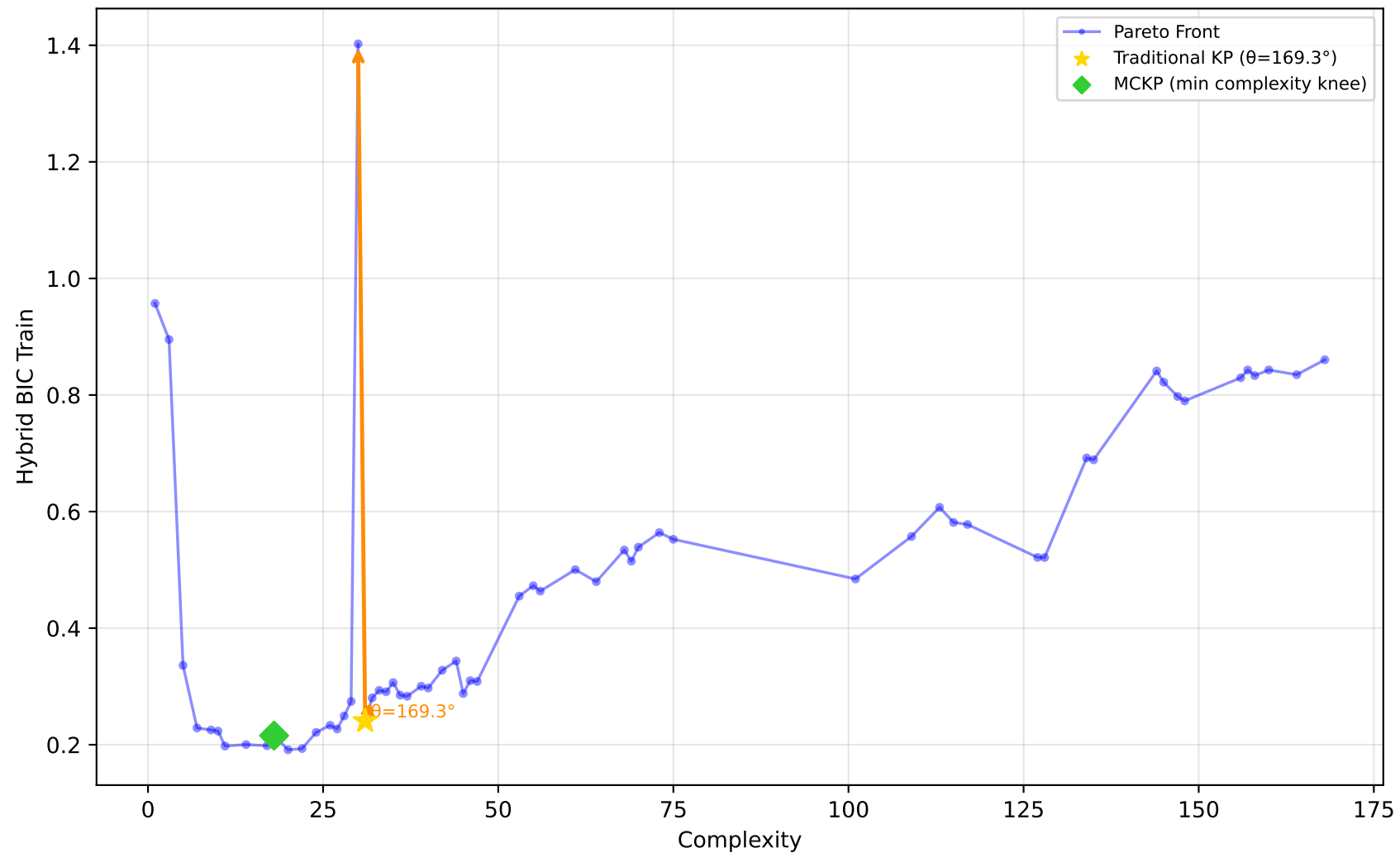
712_chscase_geyser1 - Run 6 - MVP - Hybrid BIC Train \lambda_1=0.20, \lambda_2=1.00, \lambda_3=1.00 | Difficulty: 1.00 | Method: hmr
