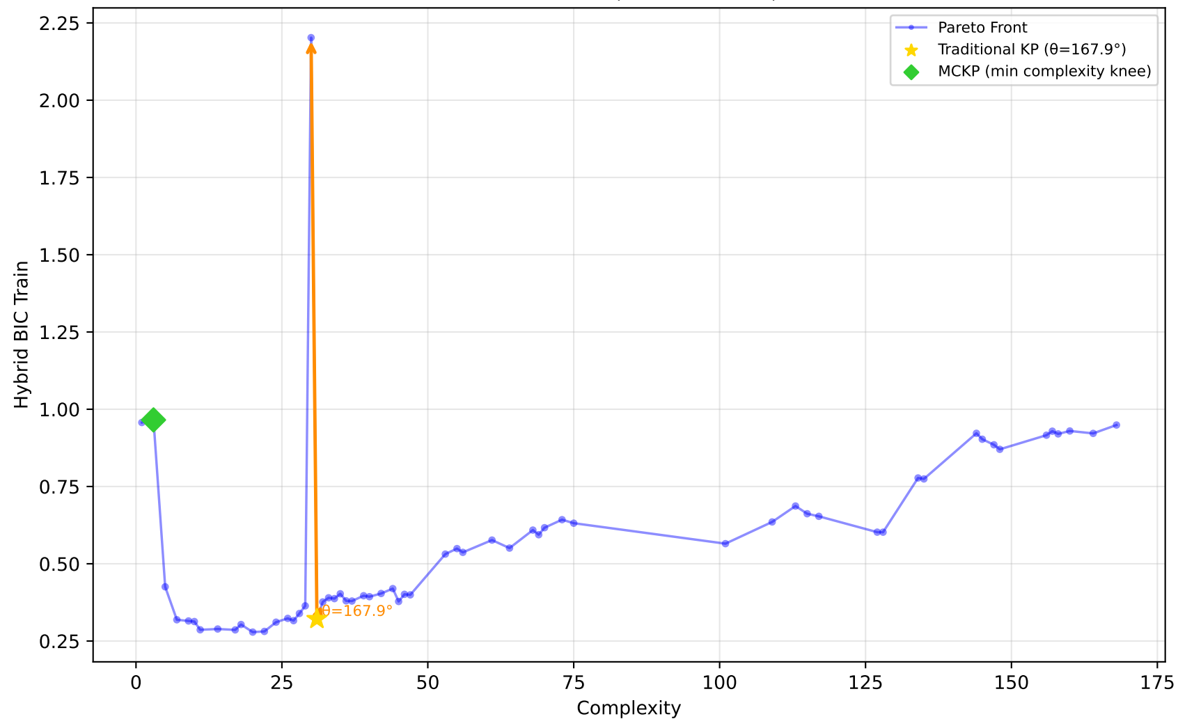
712_chscase_geyser1 - Run 6 - MVP - Hybrid BIC Train \lambda_1=1.00 , \lambda_2=1.00 , \lambda_3=1.00 | Difficulty: 1.00 | Method: hmr
