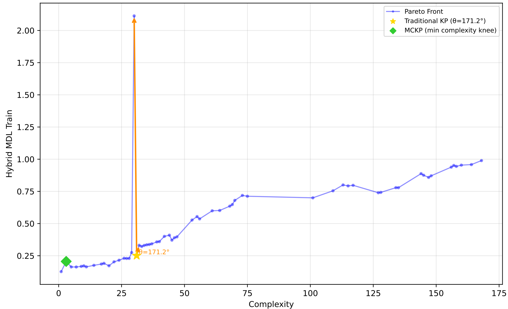
712_chscase_geyser1 - Run 6 - MVP - Hybrid MDL Train \lambda_1=1.00 , \lambda_2=1.00 , \lambda_3=1.00 | Difficulty: 1.00 | Method: hmr
