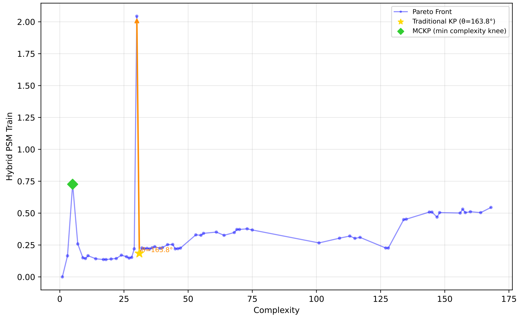
712_chscase_geyser1 - Run 6 - MVP - Hybrid PSM Train \lambda_1=1.00 , \lambda_2=1.00 , \lambda_3=1.00 | Difficulty: 1.00 | Method: hmr
