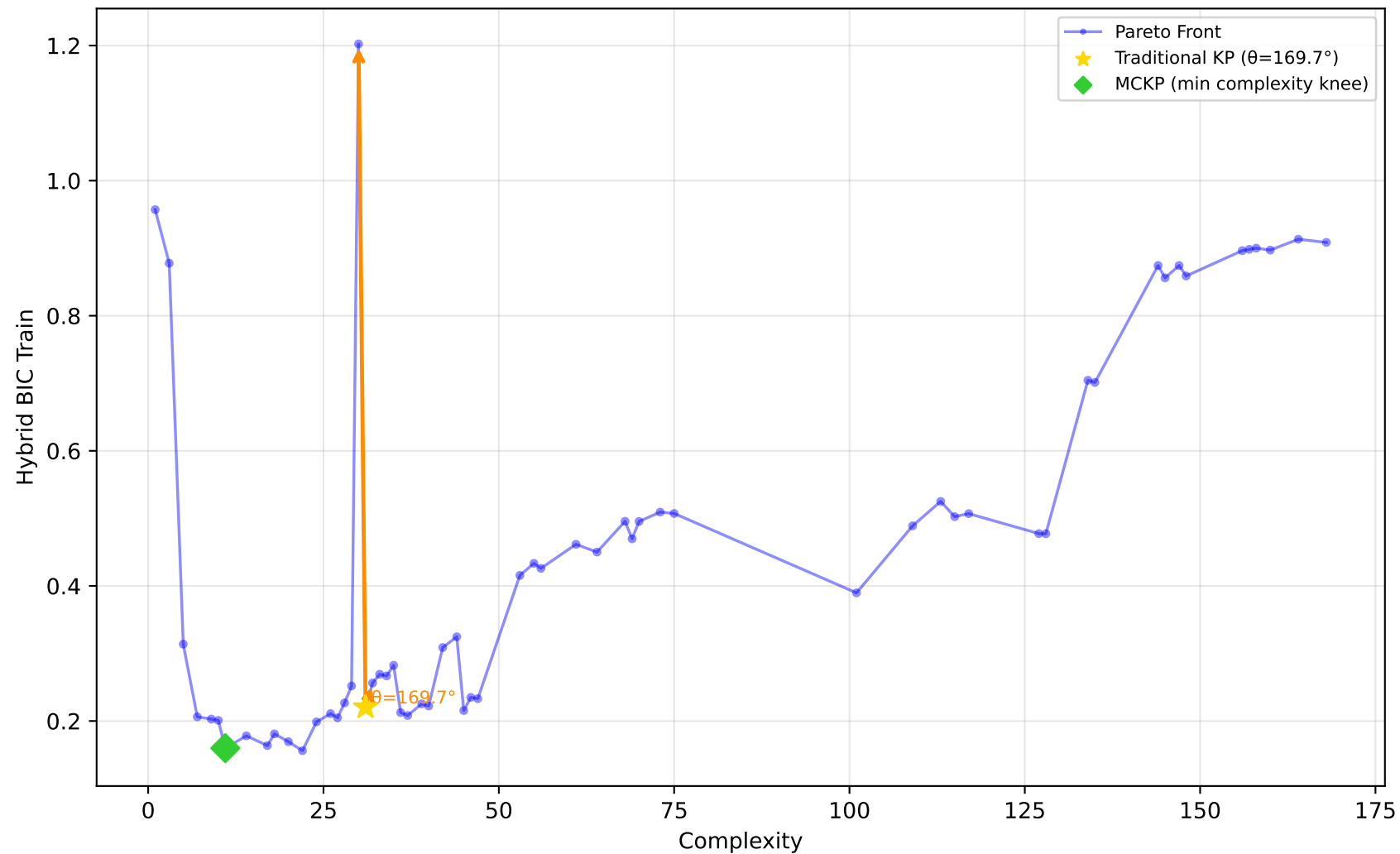
712_chscase_geyser1 - Run 6 - SVP - Hybrid BIC Train \lambda_1=0.00 , \lambda_2=1.00 , \lambda_3=1.00 | Difficulty: 1.00 | Method: hmr
