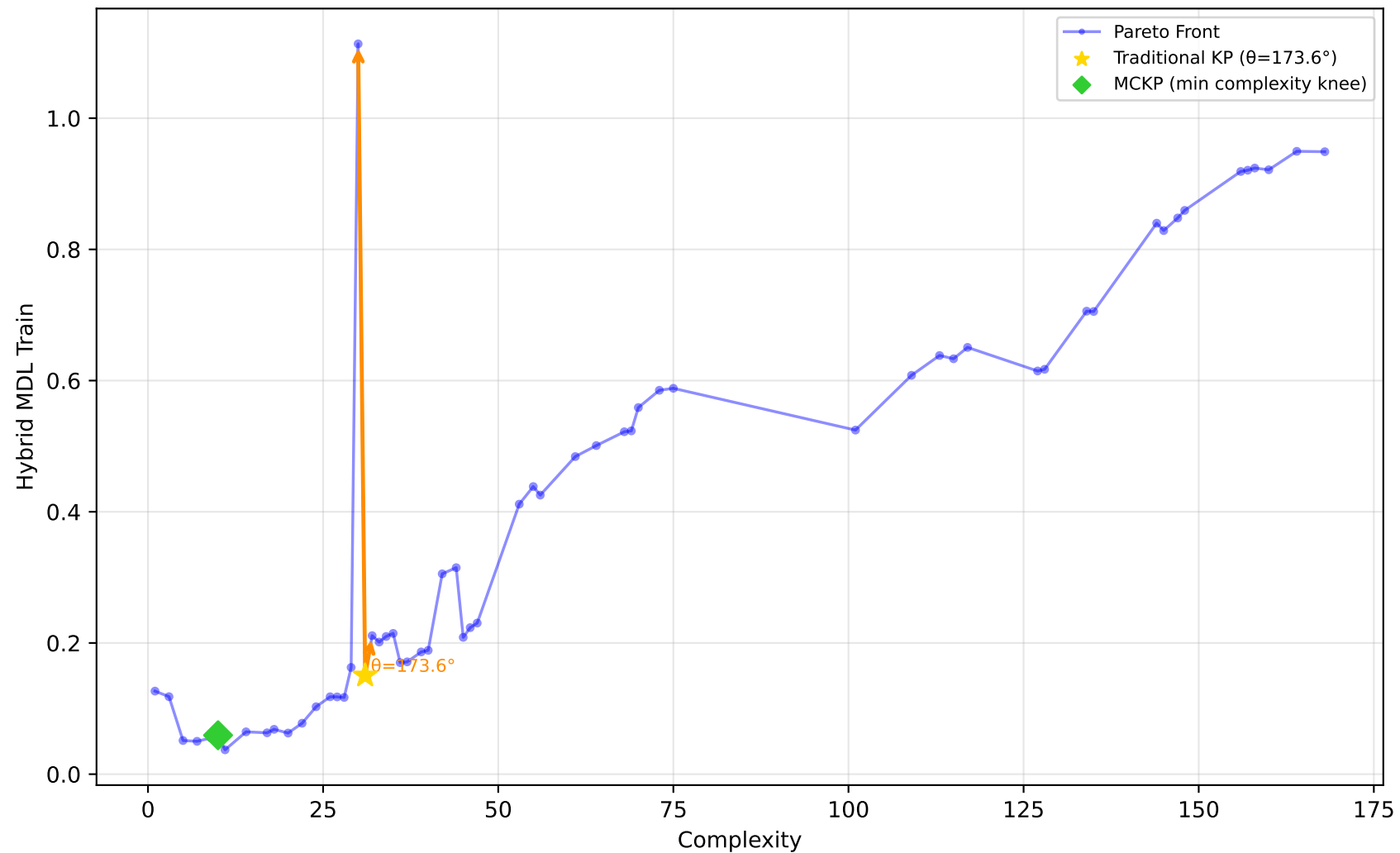
712_chscase_geyser1 - Run 6 - SVP - Hybrid MDL Train \lambda_1=0.00, \lambda_2=1.00, \lambda_3=1.00 | Difficulty: 1.00 | Method: hmr
