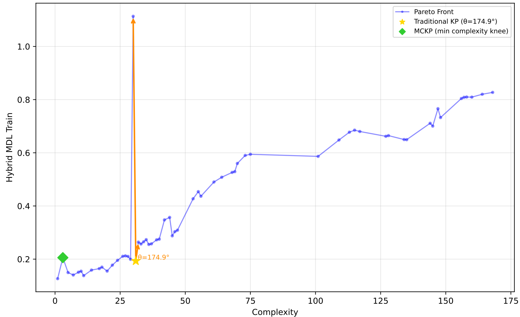
712_chscase_geyser1 - Run 6 - SVP - Hybrid MDL Train \lambda_1=1.00, \lambda_2=1.00, \lambda_3=0.00 | Difficulty: 1.00 | Method: hmr
