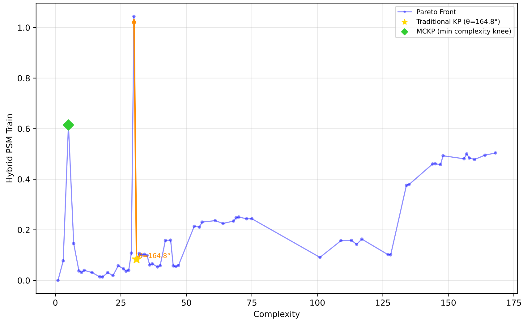
712_chscase_geyser1 - Run 6 - SVP - Hybrid PSM Train \lambda_1=0.00, \lambda_2=1.00, \lambda_3=1.00 | Difficulty: 1.00 | Method: hmr
