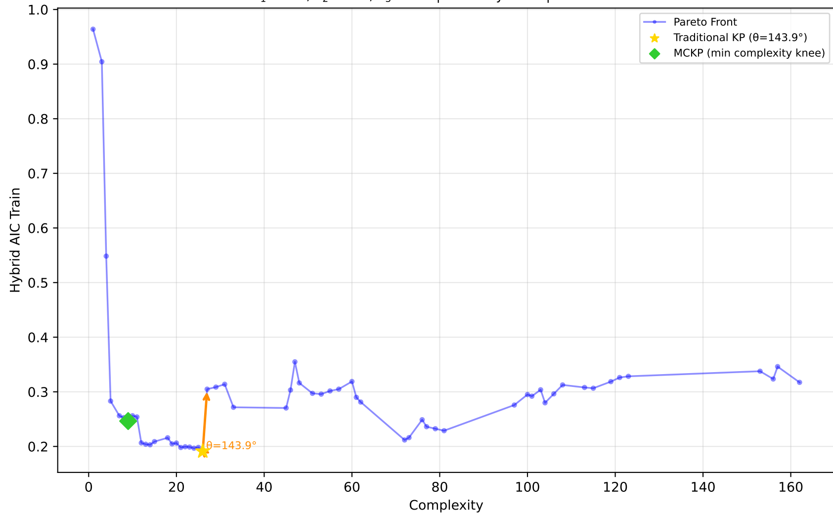
712_chscase_geyser1 - Run 7 - MVP - Hybrid AIC Train \lambda_1=0.20 , \lambda_2=1.00 , \lambda_3=1.00 | Difficulty: 1.00 | Method: hmr
