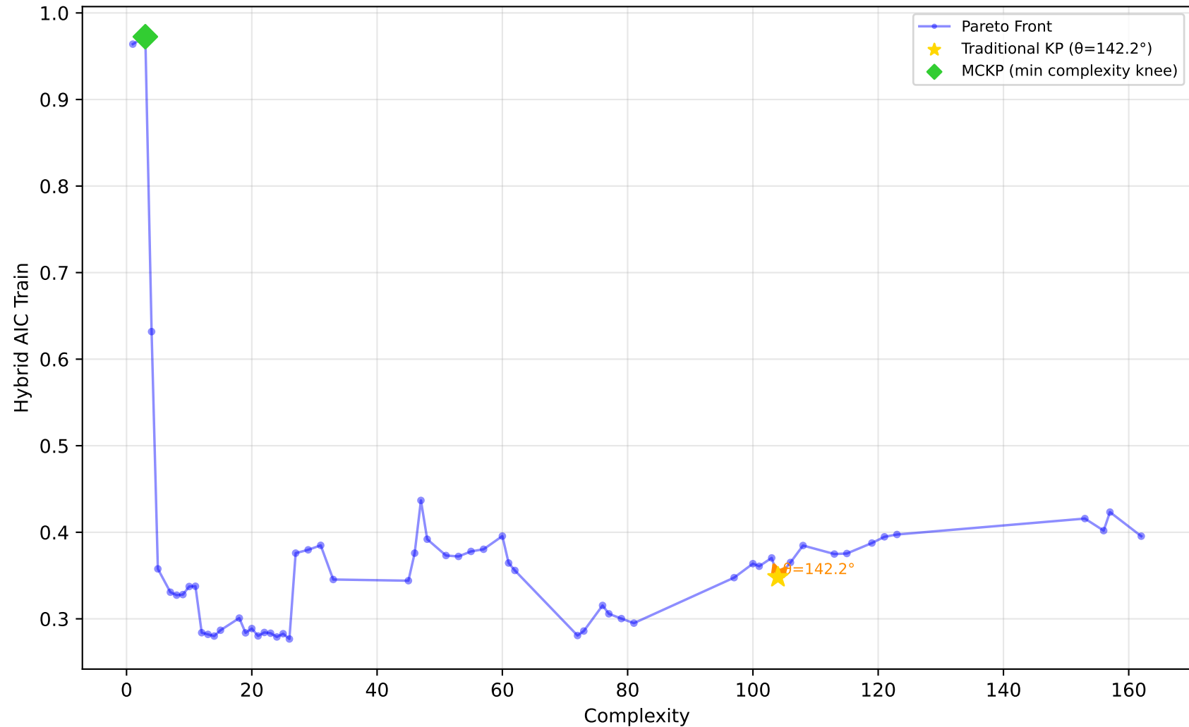
712_chscase_geyser1 - Run 7 - MVP - Hybrid AIC Train \lambda_1=1.00, \lambda_2=1.00, \lambda_3=1.00 | Difficulty: 1.00 | Method: hmr
