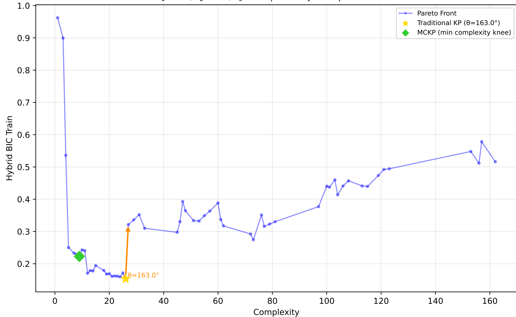
712_chscase_geyser1 - Run 7 - MVP - Hybrid BIC Train \lambda_1=0.20, \lambda_2=1.00, \lambda_3=1.00 | Difficulty: 1.00 | Method: hmr
