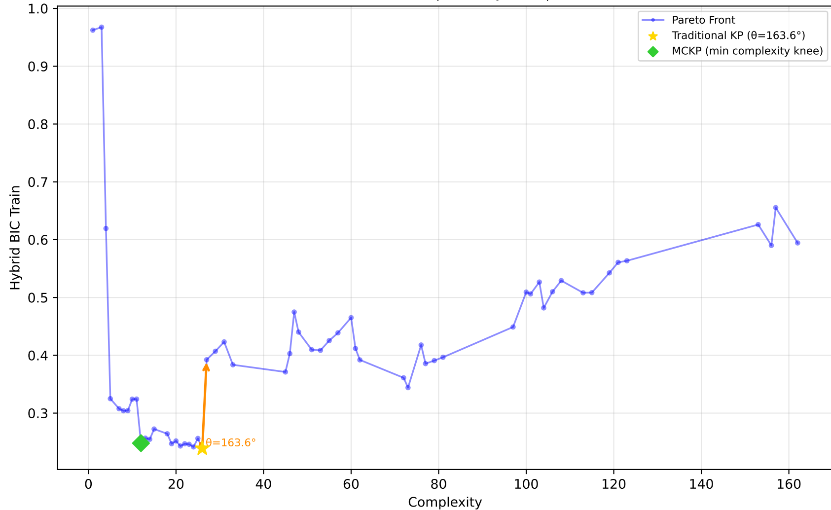
712_chscase_geyser1 - Run 7 - MVP - Hybrid BIC Train \lambda_1=1.00, \lambda_2=1.00, \lambda_3=1.00 | Difficulty: 1.00 | Method: hmr
