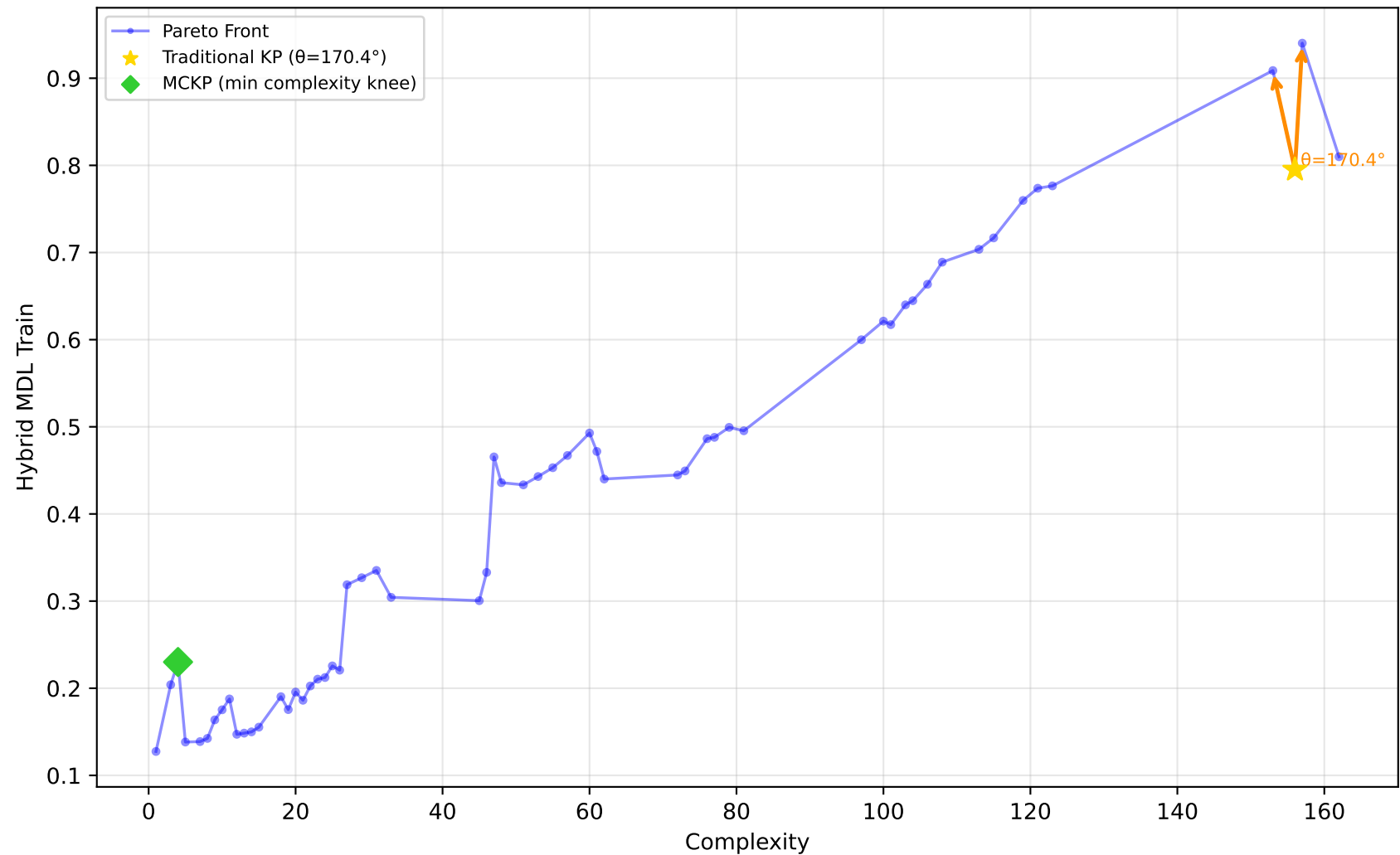
712_chscase_geyser1 - Run 7 - MVP - Hybrid MDL Train \lambda_1=1.00, \lambda_2=1.00, \lambda_3=1.00 | Difficulty: 1.00 | Method: hmr
