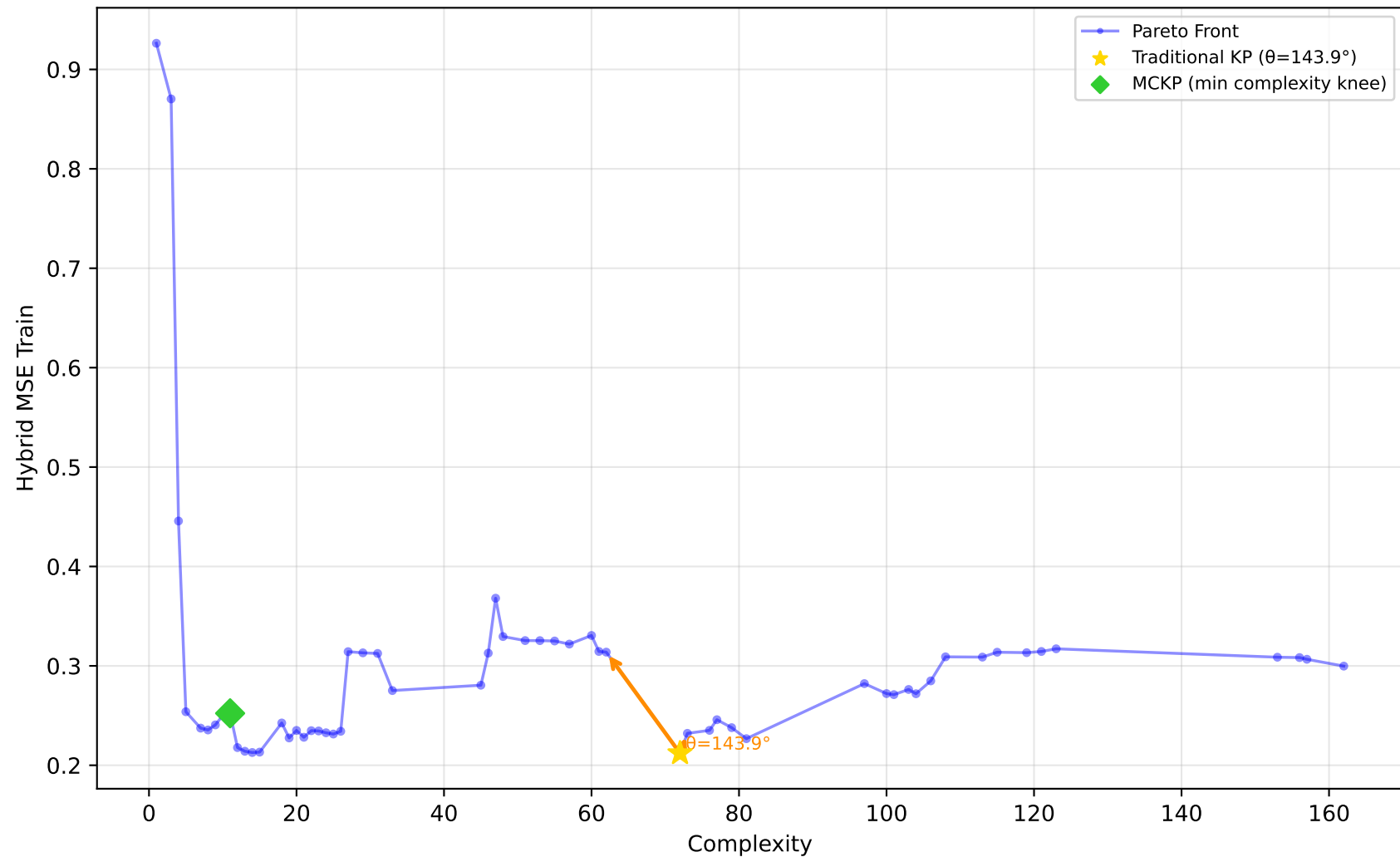
712_chscase_geyser1 - Run 7 - MVP - Hybrid MSE Train \lambda_1=1.00, \lambda_2=1.00, \lambda_3=1.00 | Difficulty: 1.00 | Method: hmr
