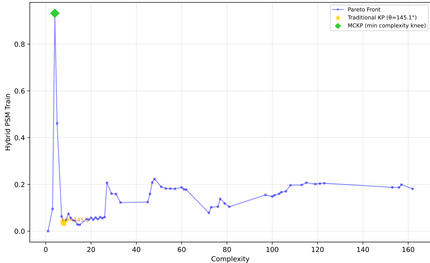
712_chscase_geyser1 - Run 7 - MVP - Hybrid PSM Train \lambda_1=0.20, \lambda_2=1.00, \lambda_3=1.00 | Difficulty: 1.00 | Method: hmr
